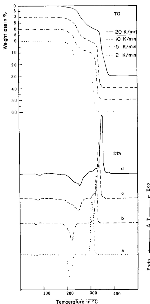
Fig. 1. TG and DTA curves of \text{NiODH} in dynamic ( 30 \text{ cm}^3 \text{ min}^{-1} ) atmosphere of air at the heating rates indicated.
