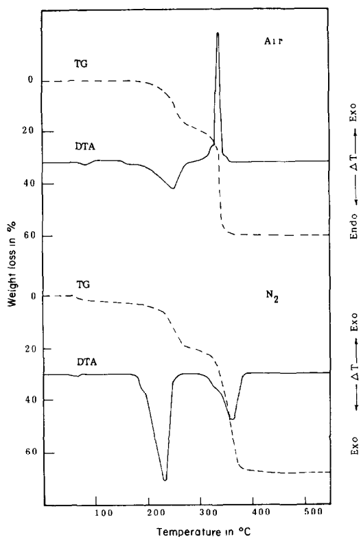
Fig. 4. The TG and DTA curves in N_2 and air ( 30 \text{ cm}^3 \text{ min}^{-1} ) at 10 \text{ K min}^{-1} .
