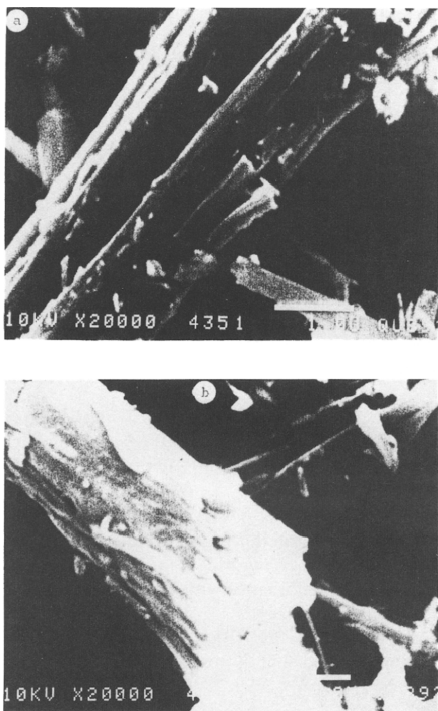
Fig. 9. (a) Scanning electron micrograph of NiODH heated at 320°C. (b) Light crushing of NiODH heated at 320°C revealed an internal slab-like structure.
