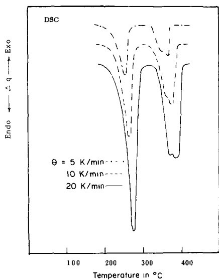
Fig. 5. DSC curves of NiODH at the heating rates ( \theta ) indicated and in dynamic ( 30 \text{ cm}^3 \text{ min}^{-1} ) atmosphere of dry nitrogen.
