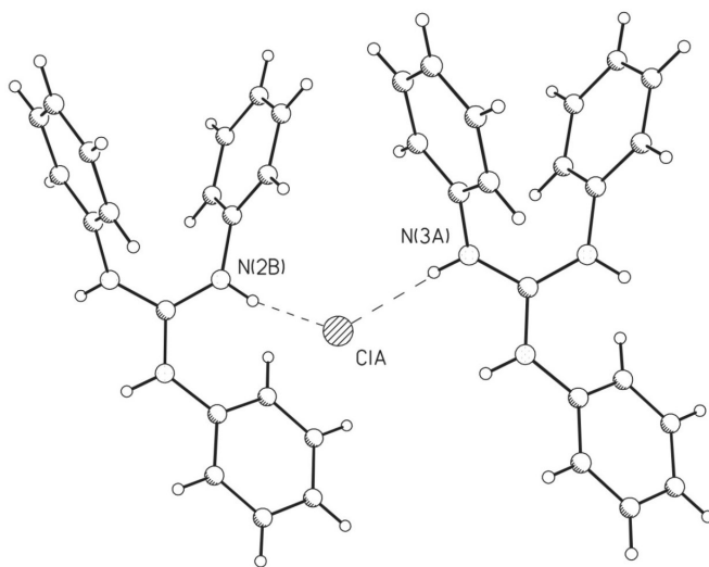
FIG. 2 Weak bonding interactions in compound 3 (thermal ellipsoids are drawn at the 50% probability level)
