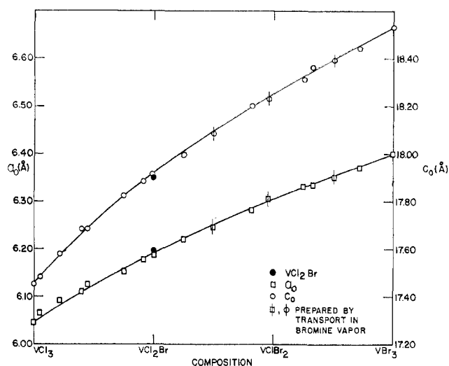
Fig. 1.—Lattice parameters of solid solutions in the system \text{VCl}_3\text{--VBr}_3 .
