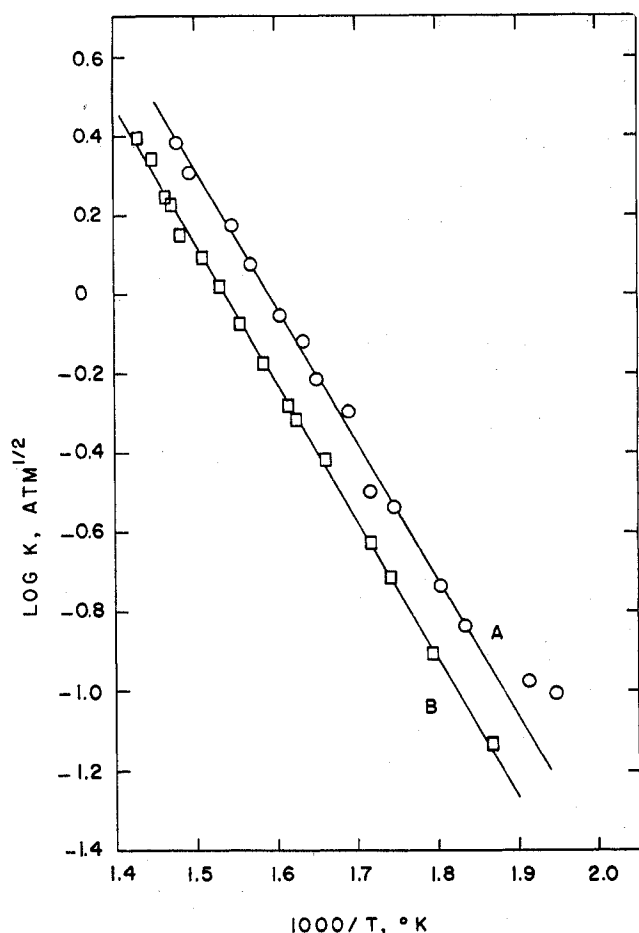
Fig. 2.—Apparent equilibrium constants for the reaction of bromine with \text{VCl}_3 and \text{VCl}_2\text{Br} : A, \text{VCl}_3 ; B, \text{VCl}_2\text{Br} .
