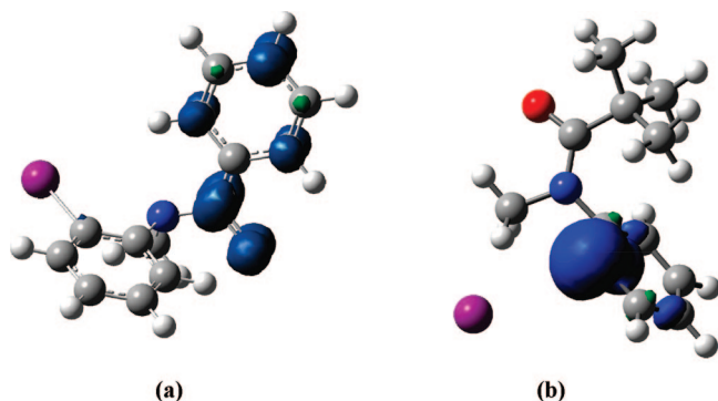
FIGURE 1. B3LYP/LANL2DZ unpaired spin density of (a) 4a •- and (b) of the charge-radical complex formed by ET to 4d , both in DMSO (density isovalue = 0.005).
