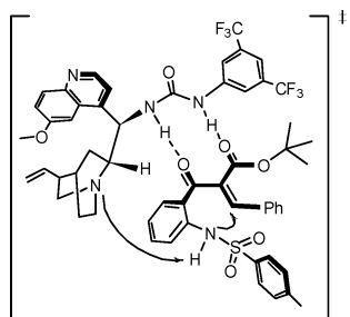
Figure 3. Proposed transition state model.
