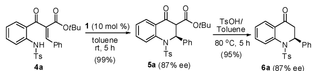
Scheme 1. Synthesis of 2-Phenyl-2,3-dihydro-4-quinolone 6a via Conjugate Addition-Decarboxylation Sequence
