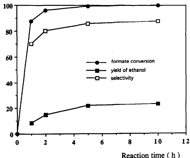
Fig. 3. Effect of initial water concentration in the synthesis of ethanol from methyl formate (conditions in Table 1).
