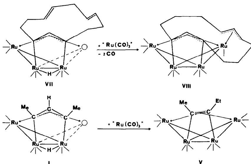
Fig. 3. Different reaction pathways of (VII) and (I) with fragments from Ru 3 (CO) 12 .
