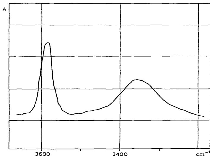
Fig. 1. Infrared spectrum of a benzene solution of \text{RhH(PPh}_3)_4 ( 2 \times 10^{-2} M ) and \text{PhCHOHCH}_3 ( 4 \times 10^{-2} M ).
