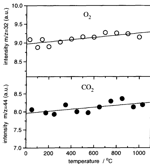
Fig. 11. Relationship between intensities of the MS signals, m/z=32 and 44, and temperature. The 1 ml pulses of oxygen and carbon dioxide were injected into the argon stream during heating with 4\text{ K min}^{-1} .
