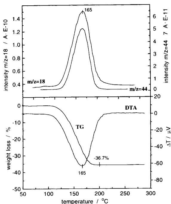
Fig. 4. Decomposition of sodium bicarbonate under argon investigated by TG, DTA and MS (simultaneous evolution of \text{H}_2\text{O} and \text{CO}_2 is monitored by the curves m/z=18 and m/z=44 , respectively).
