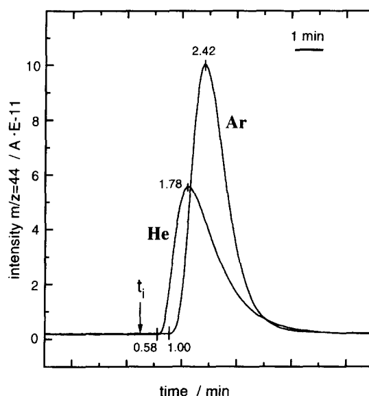
Fig. 12. Comparison of m/z=44 signals produced by injection of 1 ml of CO_2 into the streams of argon and helium (flow rate 50\text{ ml min}^{-1} ). The moment of injection is labelled on the curves as t_i , the numbers describing the beginning and maximum of the signal are expressed in minutes.
