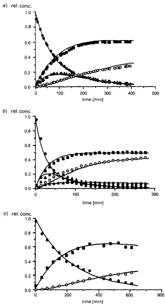
Fig. 4. Time course of the alkaline degradation of a) cefuroxime ( 1a ), b) ceftazidime ( 1b ), and c) ceftriaxone ( 1c ) in carbonate buffer solution. The continuous lines between the HPLC experimental values are the best theoretical fitting; ●: cephalosporin 1 , △: 7-epimer 2 , ■: 3-methylidene compound 3 , ○: 6-epimer 4 of 3 , ▲: \Delta^2 -cephem 5b .
