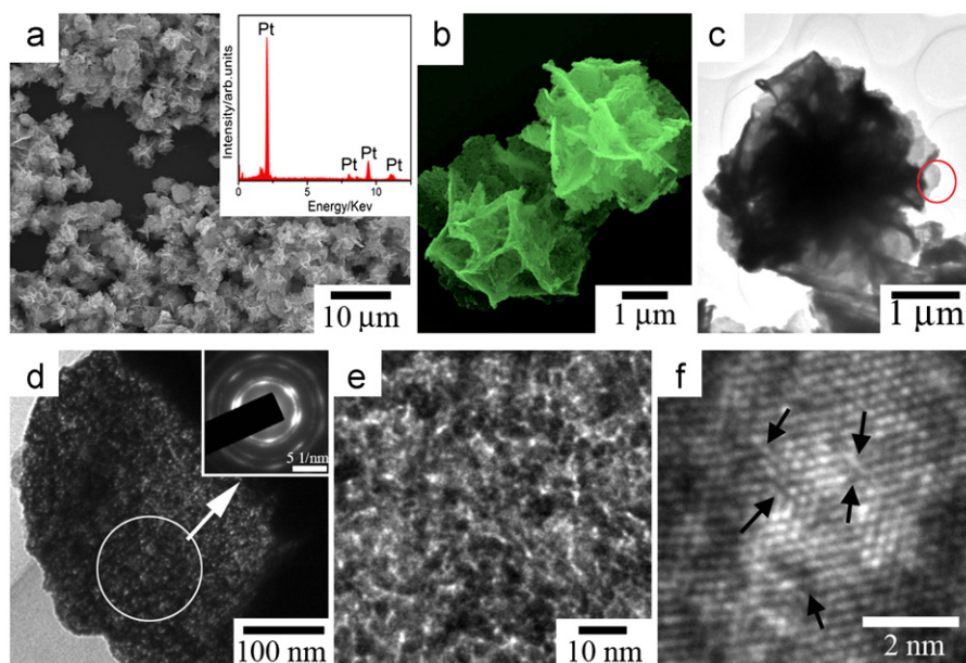
Fig. 4. SEM images of Pt MFs at low magnification (a) and high magnification (b), the inset in (a) showing the corresponding EDX pattern; TEM image of a single Pt MFs (c) and a single layer of the MF (d), the inset shows the corresponding SAED pattern (the circled part); (e) and (f) show the enlarged TEM and HRTEM images of the circled part in Fig. 2(d).
