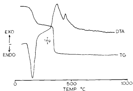
Fig. 4. Simultaneous TG and DTA curves of \text{Ni(fa)} \cdot 3\text{H}_2\text{O} . Sample mass = 11.85 mg.
