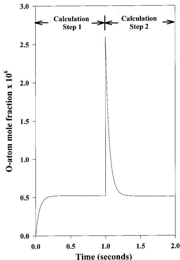
Figure 2. O atom profile for an example modeling run. The example used the standard mixture (no \text{H}_2\text{O} present) and pressure described in the text, and T = 1076 K. The k_{\text{tot}} value used is taken from ref 6. The portion from 0 to 1.0 s, a typical residence time, indicates exponential [\text{O}] increase to a constant, steady-state level due to thermal reaction of a small fraction of the \text{N}_2\text{O} during that period. Photolysis was assumed to occur at 1.0 s. The exponential decay after photolysis represents the experimentally measured quantity.
