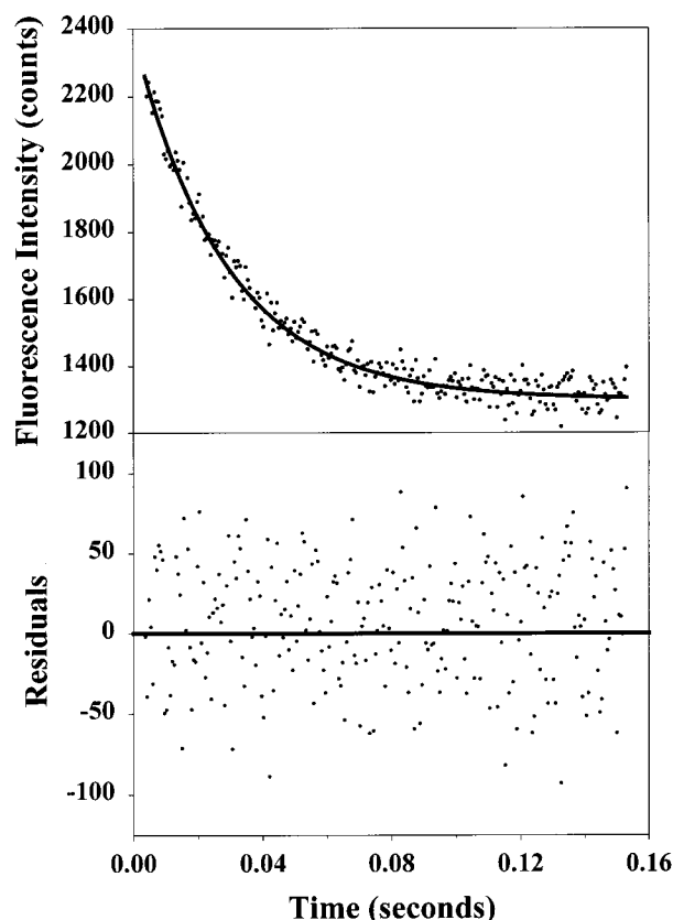
Figure 1. Example experimental [O] decay and residuals plot at 1142 K, total pressure 133 mbar, and [N 2 O] = 1.1 × 10 15 cm -3 . The fitted I_0 , k_{\text{psl}} , and B values are 1088.7, 34.67 s -1 , and 1300, respectively. Z = -0.014 . Contribution to k_{\text{psl}} due to diffusion found by fitting the ([N 2 O], k_{\text{psl}} ) data, k_d = 26 s -1 . Upper panel: measured decay (points) and fit to eq 6 (curve). Lower panel: residuals plot; a line is drawn at zero in the lower panel as an aid for visual inspection.
