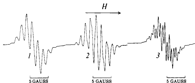
Figure 2. First derivative e.s.r. spectra of radicals 1, 2, and 3.
