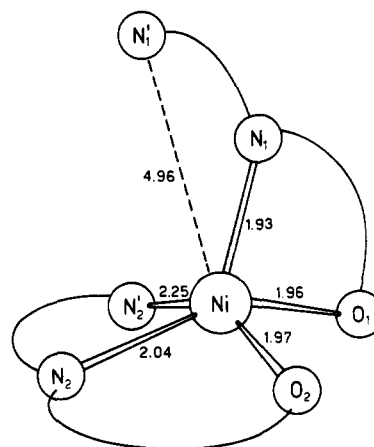
Figure 1. Sketch of the molecular structure of [\text{5-Cl-SALen-N}(\text{C}_2\text{H}_5)_2]_2\text{Ni} . Salicylaldimines residues are schematically represented by full lines.
