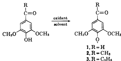
Figure 1. Oxidation of model lignin phenols. Oxidants: (a) 0.3 M \text{K}_3\text{Fe}(\text{CN})_6 in 2 M aqueous KOH; (b) 0.1 M \text{Ce}(\text{HSO}_4)_4 in 1 M aqueous \text{H}_2\text{SO}_4 ; (c) \text{PbO}_2 , solid. Solvents: benzene, toluene, and dichloromethane.
