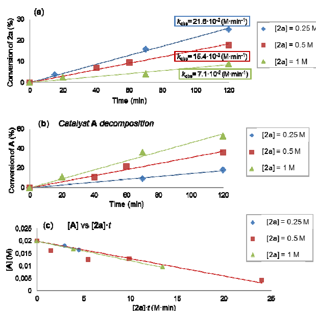
Figure 10. (a) Reaction profiles for different [2a] showing a negative-order dependence and observed rate constants. K_{obs} calculated from the slope of the plots. (b) Evolution of the catalyst concentration for the experiments in Figure 10a. We monitored the evolution of A by determining the enamine concentration in solution. (c) Overlay of plots for the kinetic data in Figure 10b according to Equation 2. Progress of the reactions followed by 1 H NMR analysis; each point corresponds to an individual run. Reactions performed in CD 3 CN under illumination by a Xenon lamp with a band-pass filter at 450 nm (irradiance = 4.7 mW/cm 2 ); [1a] 0 = 1.5 M, [A] 0 = 0.1 M; initial concentrations of 2a : 0.25 M (blue plot); 0.5 M (red plot) and 1 M (green plot). The same kinetic profiles have been observed using in situ NMR monitoring of the reaction progress, see Section I1 in the SI.
