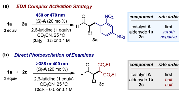
Figure 9. Model reactions used for initial-rate kinetics determined by 1 H NMR analysis and the observed rate orders. (a) EDA complex-triggered photochemical alkylation of butanal 1a with 2,4-dinitrobenzyl bromide 2a . (b) Alkylation of 1a with diethyl bromomalonate 2c driven by the direct photoexcitation of enamines. Reaction conditions: studies performed across a range of concentrations for each reaction component in CD 3 CN, irradiation at 450 and >385 nm for 2a and 2c , respectively. The kinetic studies were repeated using in situ 1 H NMR spectroscopy ( \lambda = 470 and 400 nm for 2a and 2c , respectively) to directly monitor the reaction progress. Both approaches gave similar kinetic profiles.
