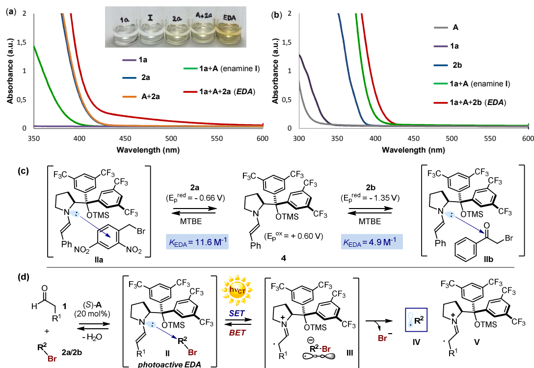
Figure 3. (a) Optical absorption spectra, recorded in MTBE in 1 mm path quartz cuvettes using a Shimadzu 2401PC UV-visible spectrophotometer, and visual appearance of the separate reaction components and of the colored EDA complex in the alkylation of 2,4-dinitrobenzyl bromide 2a ; [ 1a ] = 1.5 M; [ 2a ] = 0.5 M; [ A ] = 0.1 M. (b) Optical absorption spectra in MTBE for the alkylation with phenacyl bromide 2b ; [ 1a ] = 1.5 M; [ 2b ] = [ A ] = 0.2 M. (c) Investigating the formation of the EDA complexes in MTBE using the preformed enamine 4 ; K_{\text{EDA}} is the association constant for the EDA complex formation; E_{\text{p}}^{\text{red}} for 2a and 2b (irreversible reduction) and E_{\text{p}}^{\text{ox}} for 4 (irreversible oxidation) measured by cyclic voltammetry vs \text{Ag}/\text{Ag}^+ in \text{CH}_3\text{CN} . (d) The visible-light-triggered generation of the electrophilic carbon-centered radical IV and the \alpha -iminyl radical cation V using the enamine-based EDA complex strategy; h\nu_{\text{CT}} = charge-transfer transition energy; 16 BET = back electron transfer.
