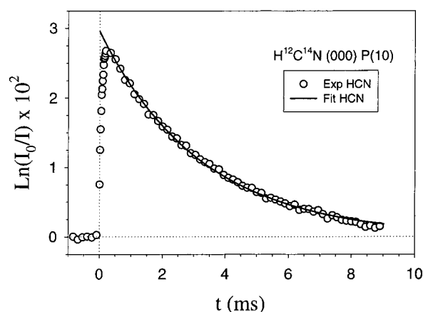
Figure 1. Typical time-resolved absorbance profile for HCN arising from reactions 2a and 3a and monitored with the \text{H}^{12}\text{C}^{14}\text{N} (000) \text{P}(10) absorption line. The circles represent experimental data. For clarity, only every third data point for 0 < t < 0.2 ms, and every 30th data point elsewhere, are shown in the plot. The solid curve is a nonlinear least-squares fit of all data for t > 0.2 ms to the simple exponential function, A\exp(-kt) , with resulting fit parameters of A = 296 and k = 308 \text{s}^{-1} . The dominant loss process for HCN is diffusion from the photolysis/probe zone. The fit extrapolation to t = 0 was used to estimate the nascent concentration of HCN from reactions 2a and 3a (see text). The experimental conditions were P_{\text{Ar}} = 2.45 , P_{(\text{CN})_2} = 0.061 , and P_{\text{CH}_3\text{SH}} = 0.023 Torr at 293 K.
