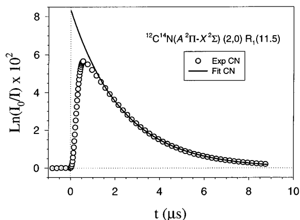
Figure 2. Typical time-resolved absorbance profile for CN arising from reaction 2 and monitored with the ^{12}\text{C}^{14}\text{N} ( A^2\Pi-X^2\Sigma ) (2,0) R_1 -(11.5) absorption line. The circles represent experimental data. For clarity, only every second data point for 0 < t < 0.5 \mu\text{s} , and every 20th data point elsewhere, are shown in the plot. The solid curve is a nonlinear least-squares fit of all data for t > 1.4 \mu\text{s} to the simple exponential function, A\exp(-kt) , with resulting fit parameters of A = 832 and k = 4.29 \times 10^5 \text{ s}^{-1} . The dominant loss process for CN is reaction 3, with a characteristic time of 2.33 \mu\text{s} . The first-order rate constant, k , from this and other experiments were used to determine the bimolecular rate constant, k_3 , for reaction 3 (see text and Figure 5). The experimental conditions were P_{\text{Ar}} = 2.40 , P_{(\text{CN})_2} = 0.084 , and P_{\text{CH}_3\text{SH}} = 0.024 Torr at 293 K.
