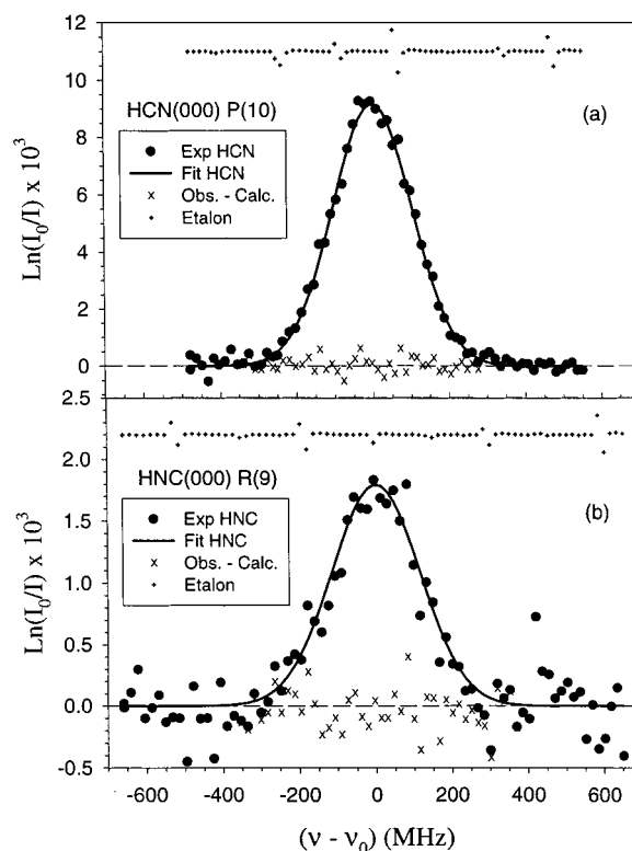
Figure 3. Typical frequency-resolved absorbance profiles for (a) HCN arising from reactions 3a and 4a and monitored with the \text{H}^{12}\text{C}^{14}\text{N} (000) P(10) absorption line, and (b) HNC arising from reactions 3b and 4b and monitored with the \text{H}^{14}\text{N}^{12}\text{C} (000) R(9) absorption line. The filled circles represent experimental data, while the solid curves are nonlinear least-squares fits to the data assuming a Gaussian line shape, with the residues indicated by the “X” symbols. The response of the 150-MHz Etalon over the scan frequency range is shown above the respective data plots in (a) and (b); the Etalon fringes from these traces were used to calibrate the probe laser frequency. The experimental conditions were P_{\text{Ar}} = 0.359 , P_{\text{C}_3\text{H}_8} = 0.958 , P_{(\text{CN})_2} = 0.060 , and P_{\text{CH}_3\text{SH}} = 0.023 Torr at 293 K, with a boxcar width of 15 \mu\text{s} centered on delays of (a) 300 \mu\text{s} and (b) 100 \mu\text{s} . At these delay times, the translational energies of the HCN and HNC products were equilibrated to the experimental temperature of 293 K.
