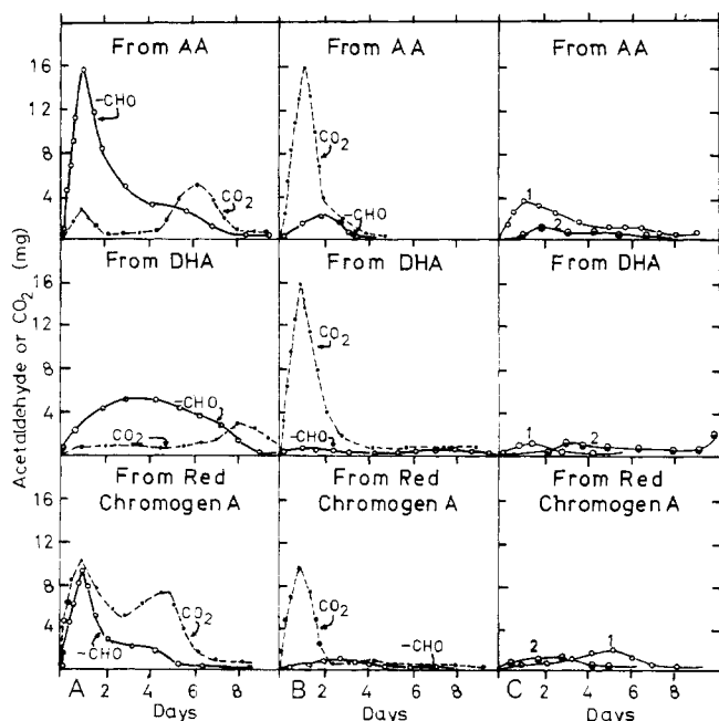
Figure 2. Formation of aldehyde and \text{CO}_2 from AA, DHA, and red chromogen A; 176 mg of AA, 174 mg of DHA, or 268 mg of red chromogen A used; acetaldehyde using alcoholic medium (1) and aqueous medium (2); (A) carrier gas, \text{O}_2 ; medium, 96% alcohol; temperature, 65^\circ ; (B) carrier gas, \text{O}_2 ; medium, aqueous; temperature, 65^\circ ; (C) carrier gas, \text{CO}_2 ; medium, 96% alcohol and aqueous; temperature, 65^\circ .
