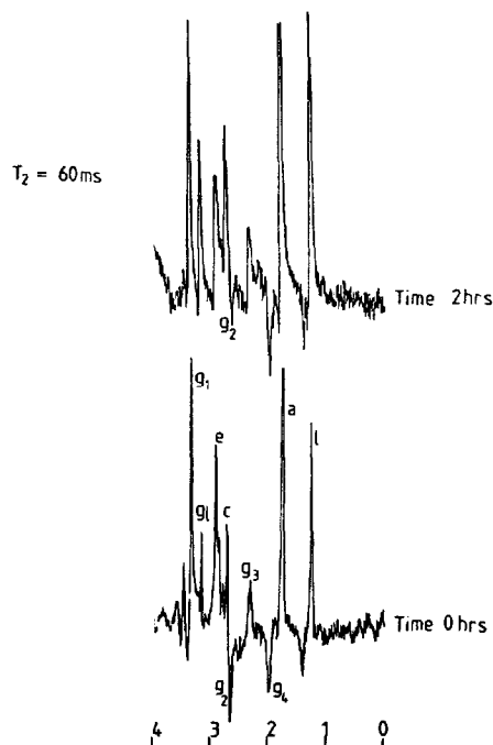
Fig. 2. The effect of 0.5 mg of sodium nitroprusside on the ^1\text{H} spin echo NMR of the human erythrocyte ( \tau = 60 ms): l, lactate; a, acetate (external reference); g1, glycine; c, creatine; e, ergothioneine; g_1 – g_4 , glutathione; the resonance assignments of glutathione and ergothioneine are shown in Fig. 1. The lower spectrum consists of 2000 scans, whereas the upper required 4000 scans (due to paramagnetism). A small presaturation pulse was applied to the water resonance.
