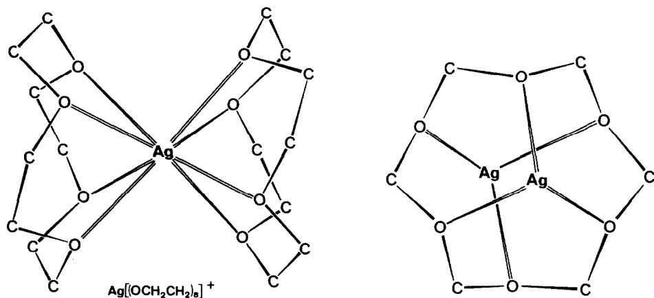
Fig. 15. Molecular structure of [Ag(OCH_2CH_2)_6]^+ AsF_6^- (the anion AsF_6^- is omitted for clarity).
