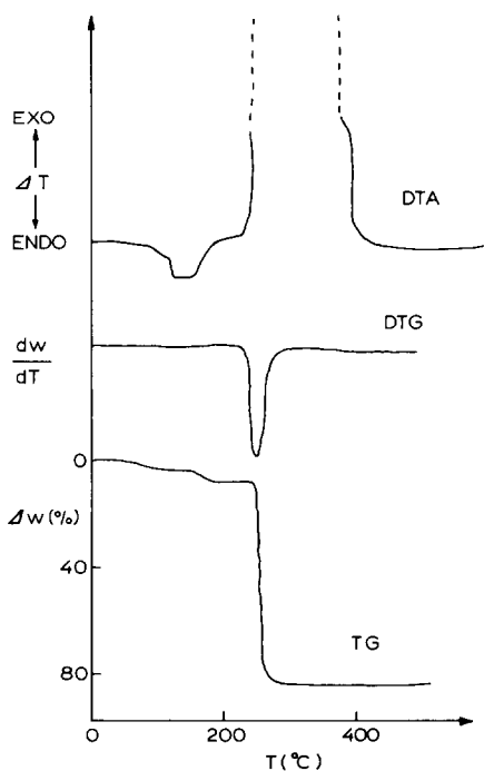
Fig. 2. TG, DTG and DTA curves for Cu(II)-5-nitrosalicylhydrazide.
