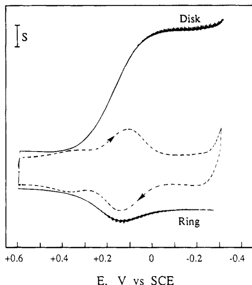
Figure 4. Current-potential curves for the catalyzed reduction of O_2 at a rotating pyrolytic graphite disk-platinum ring electrode. The disk was coated with 6 \times 10^{-10} \text{ mol cm}^{-2} of [Co^{III}P(pyRu(NH_3)_5)_4]^{13+} by spontaneous adsorption from a solution of the complex. The Pt ring electrode was maintained at 1.0 V as the disk electrode potential was scanned at 5 \text{ mV s}^{-1} . Supporting electrolyte: 0.5 M HClO_4 saturated with air. Electrode rotation rate: 100 rpm. The dashed curve is the cyclic voltammetric response of the adsorbed porphyrin in the absence of O_2 recorded at a scan rate of 50 \text{ mV s}^{-1} . Current scale: S = 10 \mu A for the disk and the dashed curve; S = 2 \mu A for the ring.
