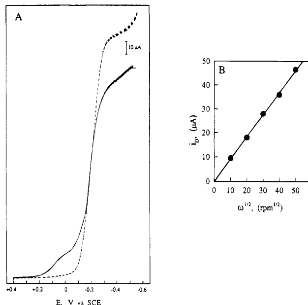
Figure 1. (A) Rotating disk voltammetry of a solution obtained from the reaction between [\text{CoP}(\text{pyH})_4]^{4+} and \text{Ru}(\text{NH}_3)_5\text{OH}_2^{2+} followed by air oxidation (solid curve). The dashed curve is the response obtained when the reaction procedure (see Experimental Section) was carried out in the absence of [\text{CoP}(\text{pyH})_4]^{4+} . Supporting electrolyte: 0.1 M \text{CF}_3\text{COOH} deaerated by bubbling with argon. Rotation rate = 100 rpm. (B) Levich plot of the plateau current for the smaller wave in (A) vs the electrode (rotation rate) 1/2 .
