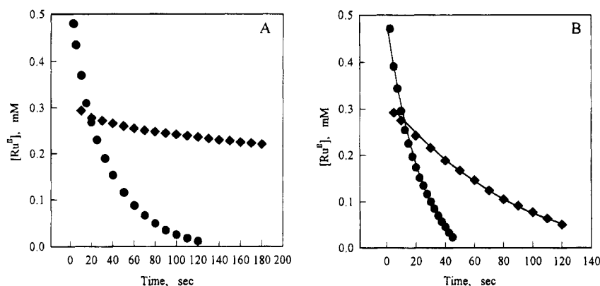
Figure 6. Kinetic data for the homogeneous reduction of O 2 by Ru(II) in the absence of a catalyst (A) or as catalyzed by 5 × 10 -6 M [CoP(pyH) 4 ] 4+ (B). Supporting electrolyte: 0.1 M CF 3 COOH continuously saturated with air; [O 2 ] = 0.28 mM. Ru(II) reductant and its initial concentration: 0.47 mM Ru(NH 3 ) 6 2+ (●); 0.31 mM Ru(NH 3 ) 5 py 2+ (◆). The points are experimental, and in (B) the lines were calculated from eq 8 using the values of k 2 , k 3 , and k 3 /k -2 given in Table 2A.
