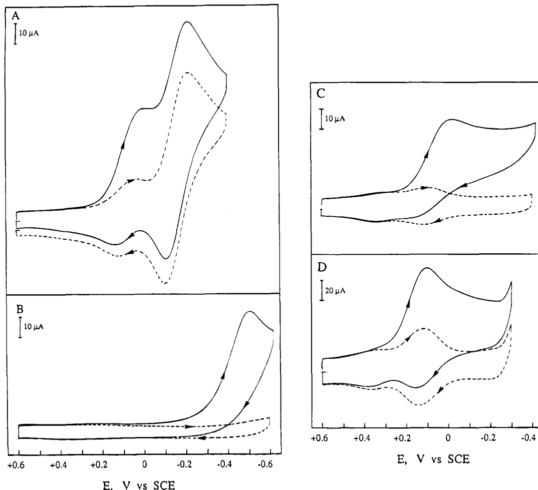
Figure 3. (A) Cyclic voltammetry of a mixture of 0.46 mM [\text{Co}^{\text{III}}\text{P}(\text{pyRu}(\text{NH}_3)_5)_4]^{13+} and 1.5 mM \text{Ru}(\text{NH}_3)_5(\text{OH}_2)^{3+} in the absence (dashed curve) and the presence (solid curve) of \text{O}_2 . Supporting electrolyte: 0.1 M \text{CF}_3\text{COOH} . Scan rate: 50 \text{ mV s}^{-1} . (B) Reduction of \text{O}_2 at an EPG electrode in pure supporting electrolyte. The dashed curve is the background response recorded in the absence of \text{O}_2 . Other conditions were as in (A). (C) Responses obtained when the electrode used to record the voltammogram in (A) was transferred to pure supporting electrolyte containing no \text{O}_2 (dashed curve) or saturated with air (solid curve). The area under the peak in the dashed curve corresponds to 9 \times 10^{-11} \text{ mol cm}^{-2} of adsorbed porphyrin. Other conditions were as in (A). (D) Repeat of (C) with an EPG electrode polished with No. 600 SiC paper instead of alumina. The quantity of porphyrin adsorbed on the electrode was 5.7 \times 10^{-10} \text{ mol cm}^{-2} .
