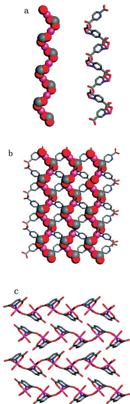
Fig. 2 (a) A space-filling view of the right-handed helical chain of -\text{C}-\text{O}-\text{Co}- and a cylindrical view of the left-handed helical chain of -\text{PDC}-\text{Co}- along the b axis. (b) The 2D structure including two types of helical chains. (c) Packing of the undulating layers along the [100] direction. The H atoms are omitted for clarity. Color code: Co: pink; C: grey; N: blue; O: red.
