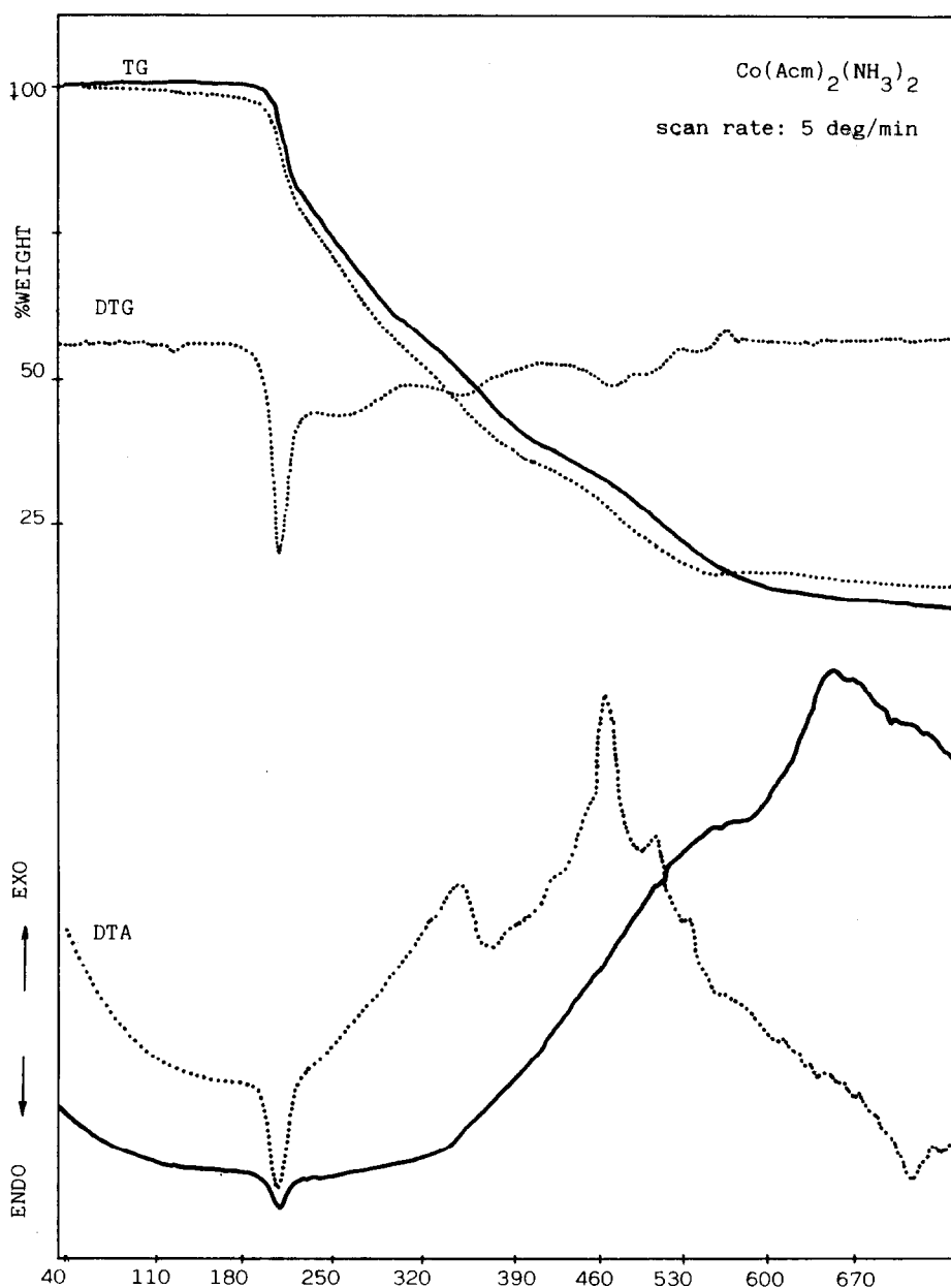
Fig. 2. \text{Co}(\text{Acm})_2(\text{NH}_3)_2 : TG/DTA curves in nitrogen (—) and in air (·····); and DTG curve in air.
