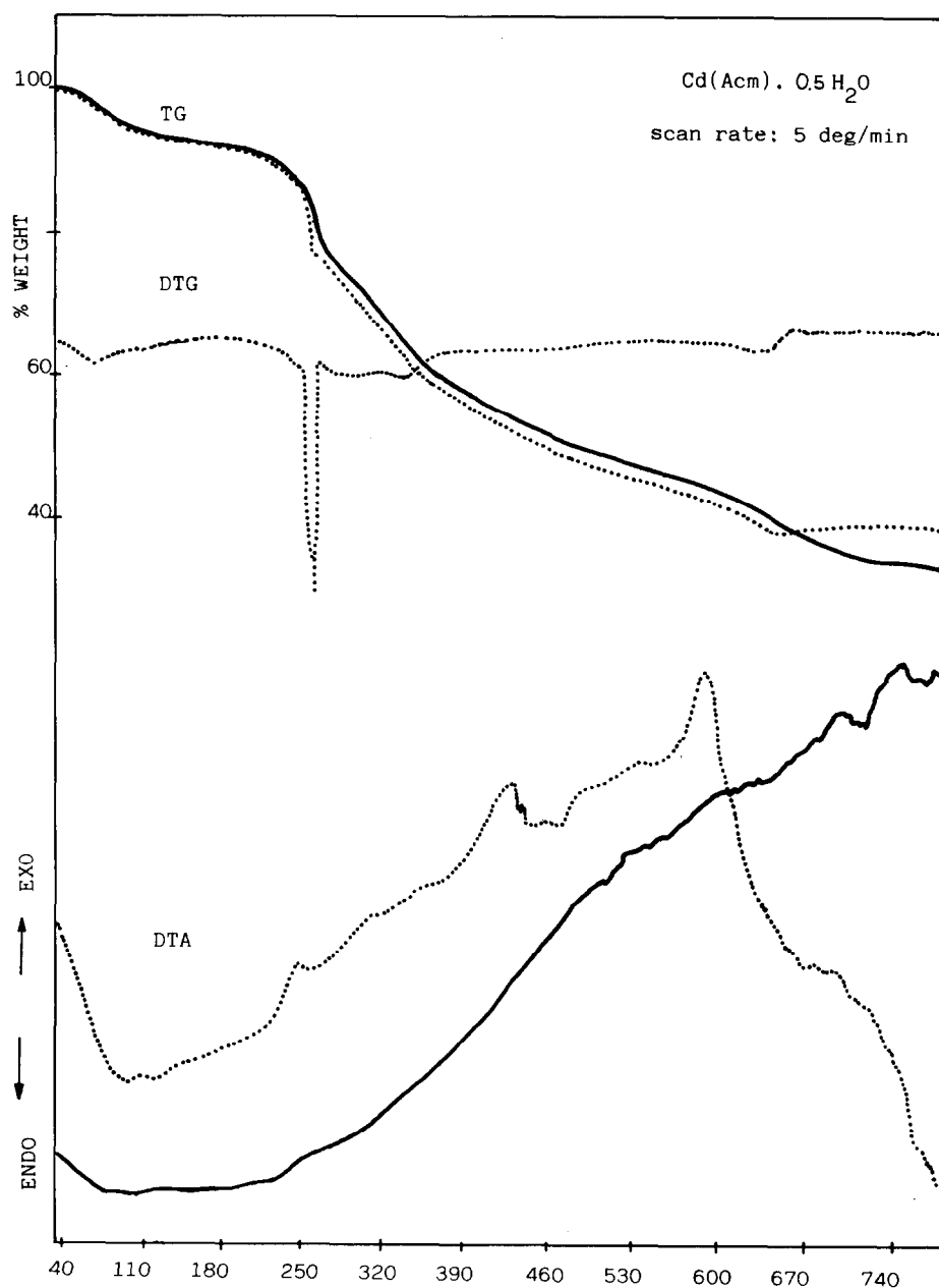
Fig. 6. \text{Cd}(\text{Acm}) \cdot 1.5\text{H}_2\text{O} : TG/DTA curves in nitrogen (—) and in air (·····); and DTG curve in air.
