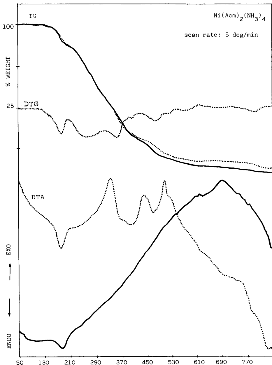
Fig. 1. \text{Ni}(\text{Acm})_2(\text{NH}_3)_4 : TG/DTA curves in nitrogen (—) and in air (·····); and DTG curve in air.
