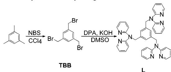
Scheme 1. Synthetic Pathway of Ligand L
