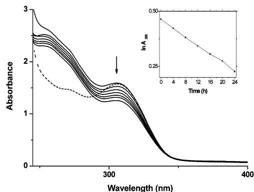
Figure 3. Time dependent absorption spectra of 3 ( 6.7 \times 10^{-5} \text{ mol} \cdot \text{L}^{-1} ) in the absence (---) and presence (—, represent 0, 4, 8, 12, 16, 20, and 24 h, respectively) of a fixed amount of CT DNA ( 1.3 \times 10^{-4} \text{ mol} \cdot \text{L}^{-1} ) at 37^\circ\text{C} . Inset shows decrease in absorbance at 305 nm ( \ln A ) with time for the reaction of 3 with DNA.
