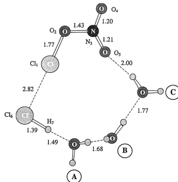
Figure 8. \text{ClONO}_2 and \text{HCl} solvated by three water molecules (cluster 1).
