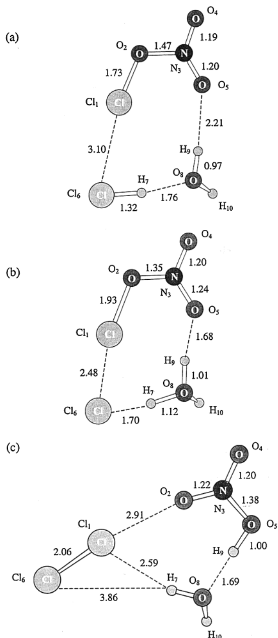
Figure 5. Stationary structures for reaction of ClONO 2 with HCl solvated by one water molecule: (a) reactants, (b) transition state, and (c) products (Cl 2 /HONO 2 ).
