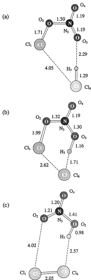
Figure 4. Stationary structures for reaction of \text{ClONO}_2 with \text{HCl} : (a) reactants, (b) transition state, and (c) products ( \text{Cl}_2/\text{HONO}_2 ).
