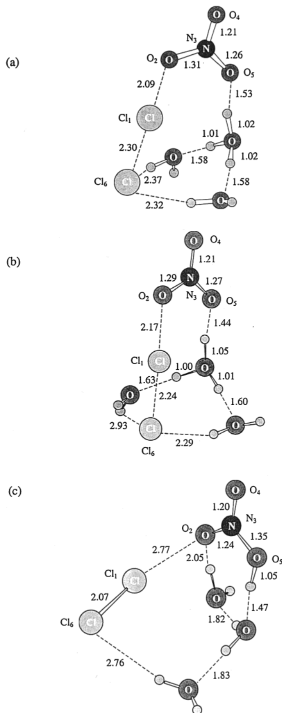
Figure 10. Stationary structures for reaction of ClONO 2 with ionized HCl solvated by three water molecules: (a) reactants (cluster 4), (b) transition state, and (c) products (Cl 2 /HONO 2 ).
