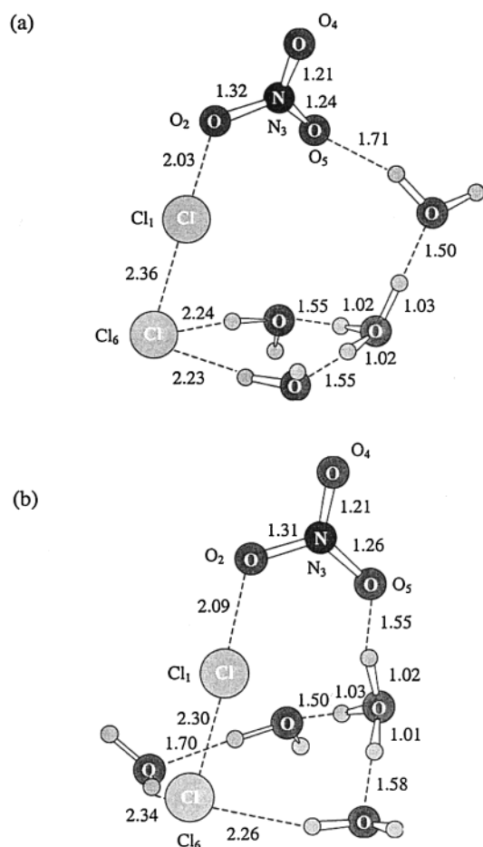
Figure 11. ClONO 2 and ionized HCl solvated by four water molecules: (a) reactant structure (cluster 5) and (b) reactant structure (cluster 6).
