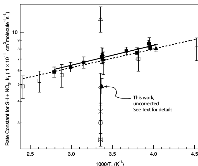
Figure 6. Arrhenius plot showing the measured values of k_1 vs 1000/T . The solid points are from this work; the squares were measured with CH 3 SH photolysis as the SH source. The solid triangles used H 2 S as the SH source. Studies of previous data from Wang et al. on k_1 are shown as open squares. The 298 K data from previous studies are the following: open triangle, Schoenle et al. (corrected by Schindler and Benter); open diamond, Stachnik and Molina; ×, Black; open circle, Friedl et al.; bow tie, Bulatov et al.
