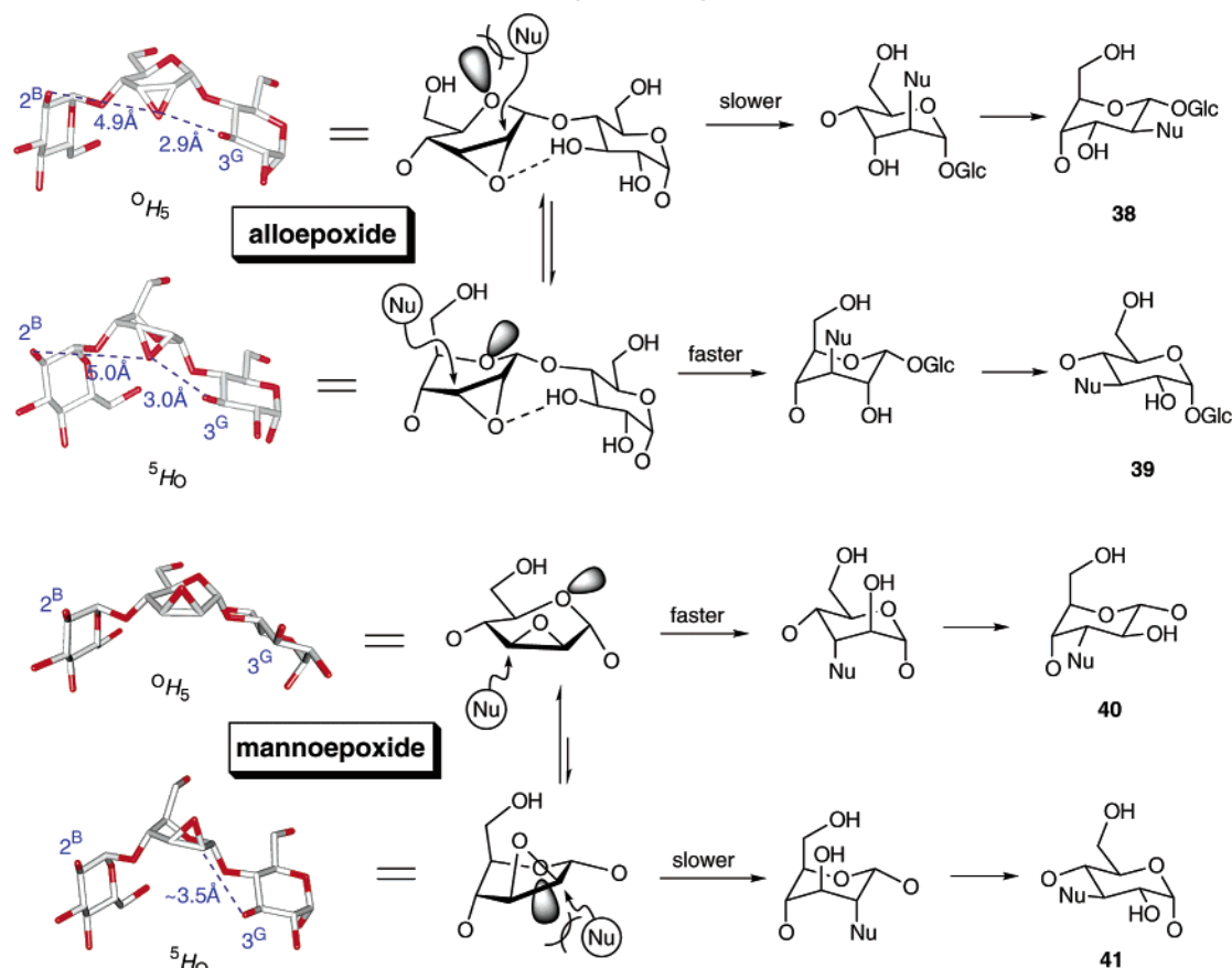
SCHEME 7. Mechanistic Consideration of the Ring-Opening Reactions of CD Epoxides a
