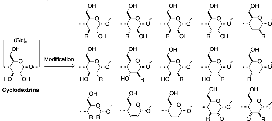
SCHEME 1. Some of the Various Subunit Structures That Can Be Potentially Derived from the Modification of the Secondary Face of CDs
