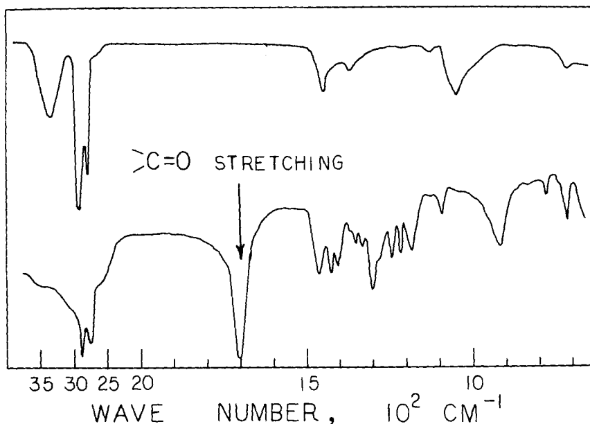
FIG. 5. — Infrared spectra of dodecenoic-2,3- ^3\text{H} , ^3\text{H} acid (lower) and dodecanol-2,3- ^3\text{H} , ^3\text{H} .
