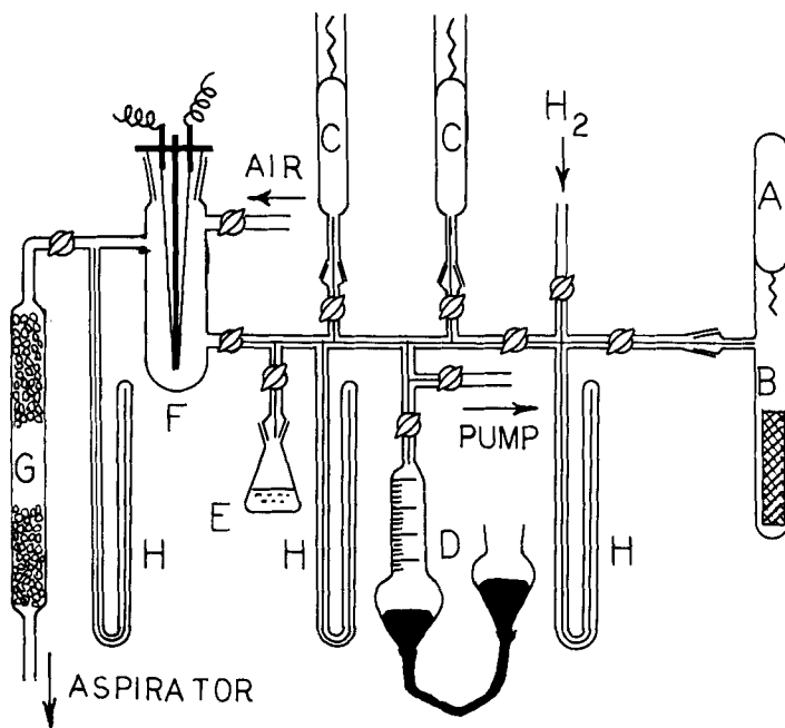
FIG. 1. — Tritiation apparatus.
