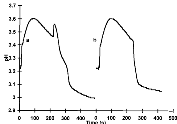
Figure 2. Chlorite-thiourea batch reactions when left in contact with air (a) and when protected (b). [H^+]_0 = 6.00 \times 10^{-4} M; [thiourea]_0 = 9.00 \times 10^{-4} M; [ClO_2^-]_0 = 2.50 \times 10^{-3} M.
