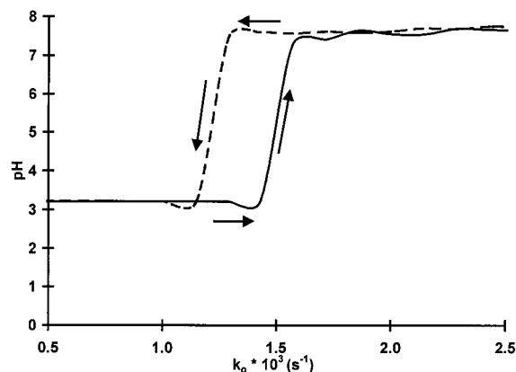
Figure 4. Simulated bi-stability. Hysteresis between a low-pH and a high-pH steady state as the flow rate is varied in both directions. [H^+]_0 = 5.00 \times 10^{-4} M; [S(-II)]_0 = 4.00 \times 10^{-4} M; [ClO_2^-]_0 = 0.02 M.
