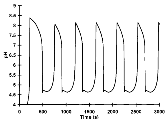
Figure 7. Simulated complex oscillations in a CSTR. [H^+]_0 = 5.00 \times 10^{-4} M; [S(-II)]_0 = 4.00 \times 10^{-3} M; [OX]_0 = 0.02 M; k_o = 1.20 \times 10^{-3} \text{ s}^{-1} .
