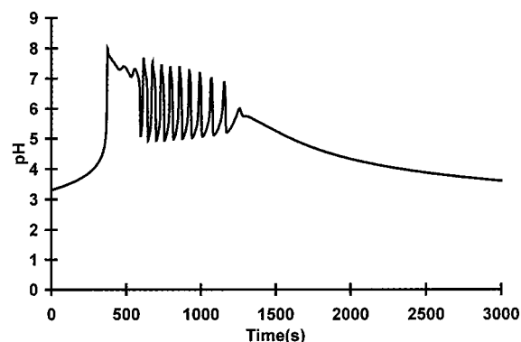
Figure 6. Simulated batch oscillations. [H^+]_0 = 5.00 \times 10^{-4} M; [S(-II)]_0 = 4.00 \times 10^{-3} M; [OX]_0 = 0.02 M.
