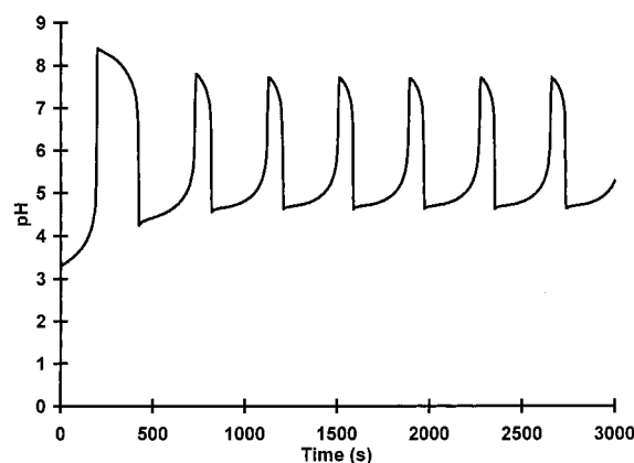
Figure 5. Simulated simple oscillations in a CSTR. [H^+]_0 = 5.00 \times 10^{-4} M; [S(-II)]_0 = 4.00 \times 10^{-4} M; [OX]_0 = 0.02 M; k_o = 4.00 \times 10^{-4} \text{ s}^{-1} .
