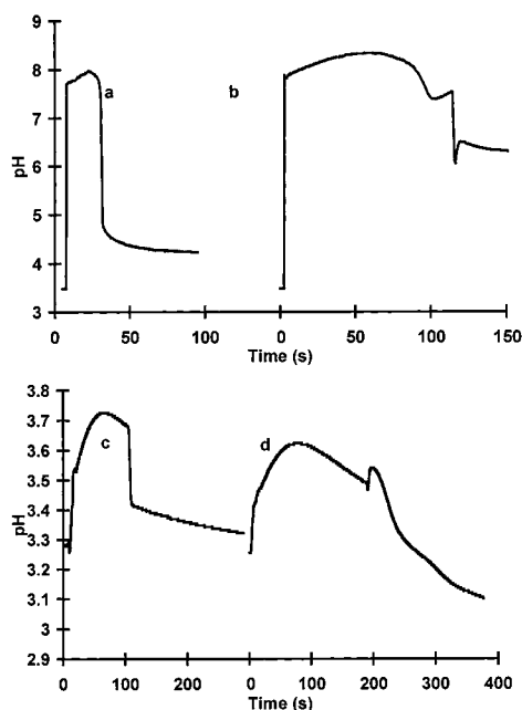
Figure 1. Measured pH vs time curves for the chlorite-sulfide (a and b) and chlorite-thiourea (c and d) systems. Chlorite-sulfide: [H^+]_0 = 3.28 \times 10^{-4} M; [S^{2-}]_0 = 7.25 \times 10^{-4} M; [ClO_2^-] = 6.13 \times 10^{-3} M (a), 6.03 \times 10^{-3} M (b). Chlorite-thiourea; [H^+]_0 = 6.00 \times 10^{-4} M; [thiourea]_0 = 9.00 \times 10^{-4} M; [ClO_2^-] = 3.00 \times 10^{-3} M (c), 2.00 \times 10^{-3} M (d).
