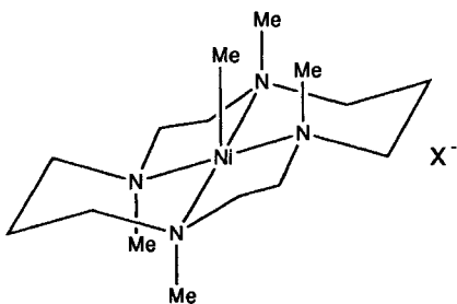
3 [\text{Ni}^{\text{II}}(\text{methyl})(\text{tmc})]^+
