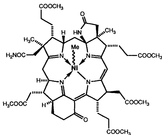
4 \text{CH}_3\text{-F430M}^{\text{II}}
