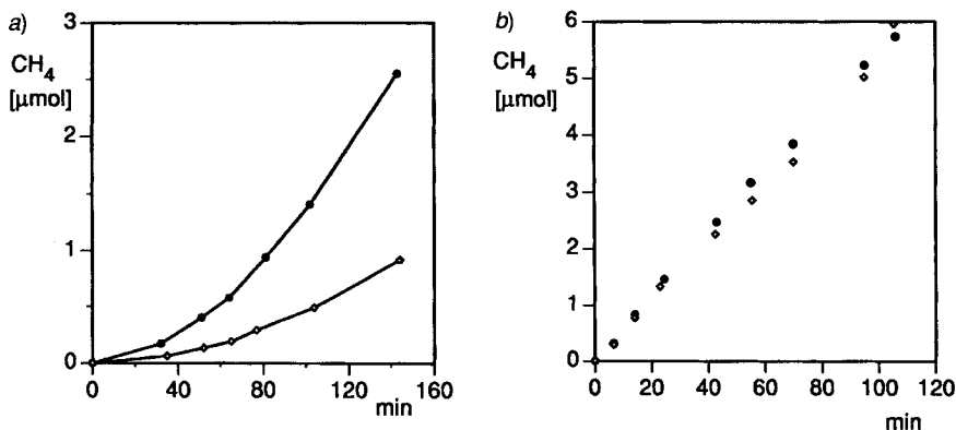
Fig. 3. Kinetic isotope effect on the rate of methane formation observed in the presence of a) i\text{-PrOD} (●) vs. i\text{-PrOH} (◇) and b) \text{PrSH} (●) vs. \text{PrSD} (◇). Conditions: see Exper. Part.
