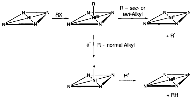
Scheme 6
