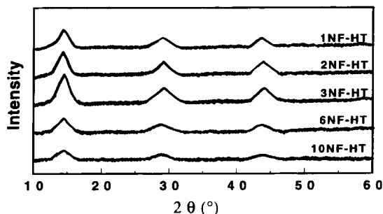
Fig. 1. XRD patterns of the Ni–Fe hydrotalcites with Ni/Fe molar ratios of 1, 2, 3, 6 and 10.
