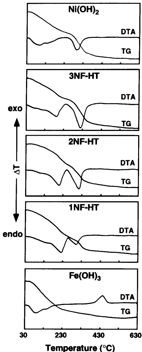
Fig. 2. TG–DTA profiles of the Ni–Fe hydrotalcites, \text{Ni}(\text{OH})_2 and \text{Fe}(\text{OH})_3 .
