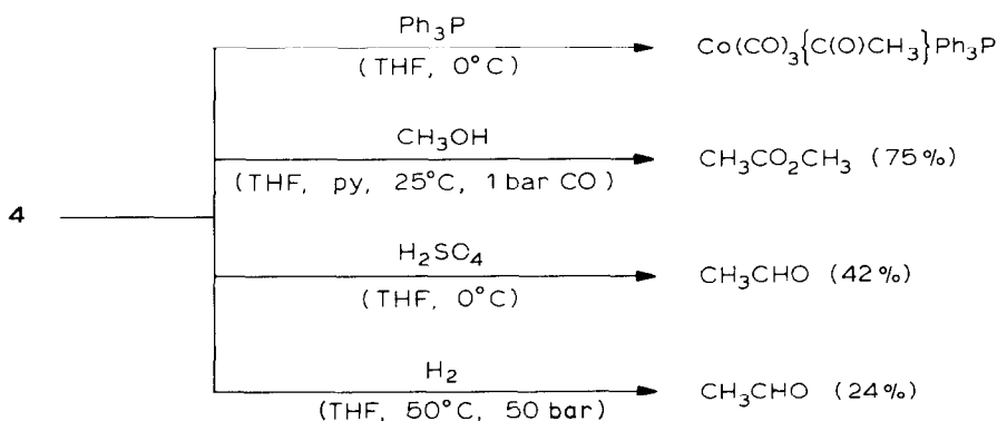
SCHEME 1. Stoichiometric model reactions with the anionic complex 4 .
