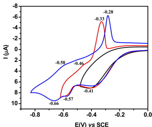
Figure 9. Cyclic voltammograms of 2 in \text{CH}_3\text{CN} containing 0.1 M [(n\text{-Bu})_4\text{N}]\text{ClO}_4 as a supporting electrolyte at 298 K, at a platinum working electrode, at a scan rate of 50 mV \text{s}^{-1} , using SCE as the reference electrode.
