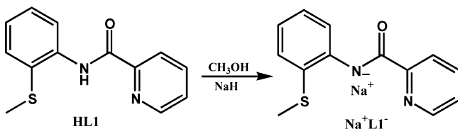
Scheme 2. Chemdraw Depiction of Ligand HL1 and Deprotonated Na + L1 –
