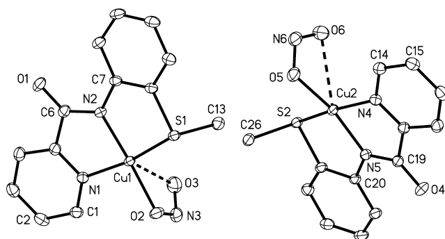
Figure 2. Thermal ellipsoid (probability level = 50%) plot of [(L1)Cu(ONO)] ( 2 ), along with the atom labeling scheme. H atoms are omitted for the sake of clarity. O3 and O6 occupy axial positions.
