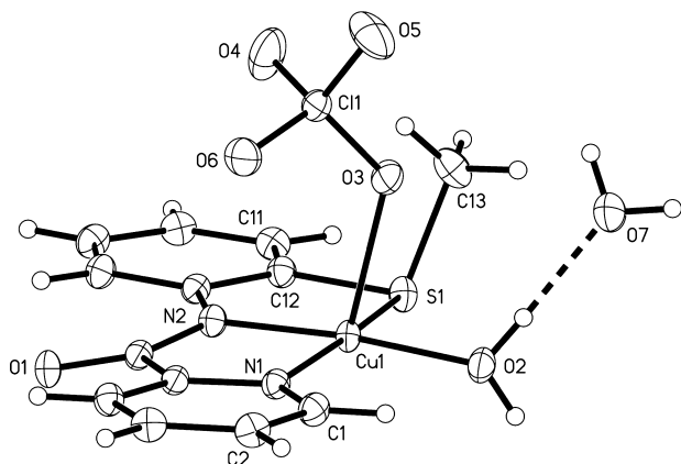
Figure 3. Thermal ellipsoid (probability level = 50%) plot of [(L1)Cu(H_2O)](ClO_4) \cdot H_2O ( 3 · H 2 O ), along with the atom labeling scheme.
