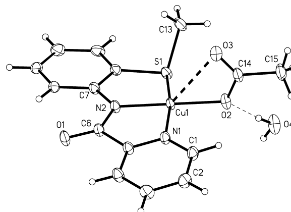
Figure 5. Thermal ellipsoid (probability level = 50%) plot of [(L1)Cu(CH_3CO_2)] \cdot H_2O ( 5 · H 2 O ), along with the atom labeling scheme.
