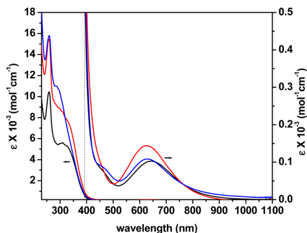
Figure 6. Electronic absorption spectra of 1 (black), 4 (blue), and 5 (red) in CH 3 OH.
