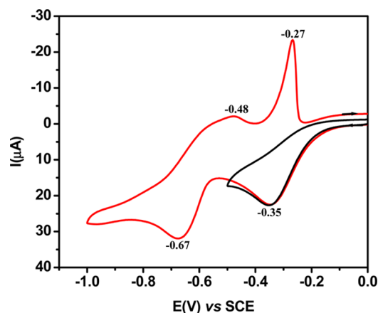
Figure 8. Cyclic voltammograms of 1 in CH 3 CN containing 0.1 M [( n -Bu) 4 N]ClO 4 as a supporting electrolyte at 298 K, at a platinum working electrode, at a scan rate of 50 mV s −1 , using SCE as the reference electrode.
