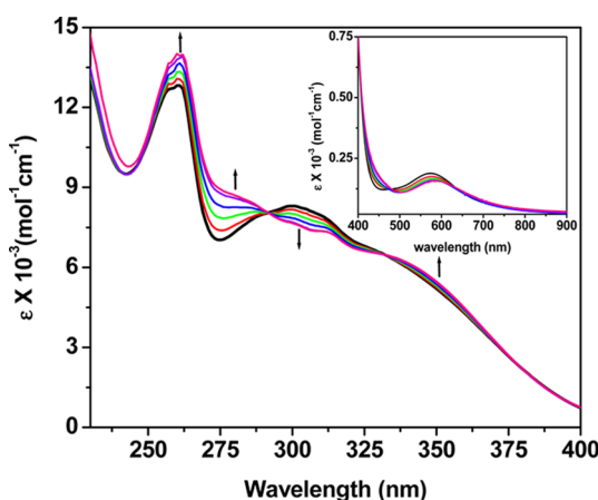
Figure 7. Electronic absorption spectral changes during transformation of 3 (black trace) → 2 (pink trace) when titrating a CH 3 CN solution of 3 with a CH 3 CN solution of ( n -Bu 4 N)NO 2 .
