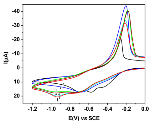
Figure 11. Cyclic voltammograms in \text{CH}_3\text{CN} containing 0.1 M [(n\text{-Bu})_4\text{N}]\text{ClO}_4 as a supporting electrolyte at 298 K, at a platinum working electrode at a scan rate of 300 \text{mV s}^{-1} , using SCE as a reference electrode: of 2 (0.96 mmol solution, black trace, a), gradual development of 0.93 V response (traces b \rightarrow e) upon coulometric reduction, followed by \text{CH}_3\text{CO}_2\text{H} reaction, after \text{N}_2 purging for 2 min (blue trace, f).
