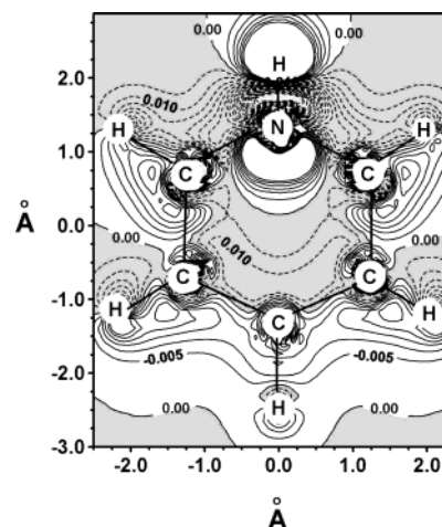
Figure 4. Electron density difference map, on the molecular plane, between pyridine and the pyridinium cation: \Delta\rho = \rho_{\text{Py}} - \rho_{\text{Py-H}^+} . Electron density in atomic units (e/bohr 3 ). Interval between isodensity lines 0.015 e/bohr 3 . Data obtained from the fully optimized results. Because the nuclear positions do not match exactly in both molecules, the results around the nuclear positions must be considered semiquantitative. Positive values (shadowed zone) indicate higher electron density in pyridine, whereas negative values correspond to a higher electron density in the pyridinium cation.
