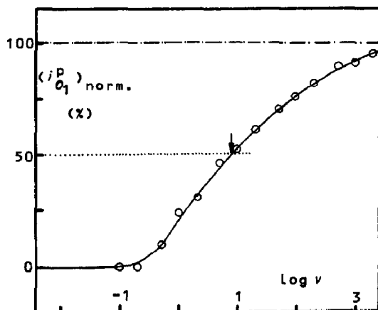
Fig. 2. Variations of the normalized current peak of wave O_1 ( (i_{O_1}^p)_{\text{norm.}} = 100 \times i_{O_1}^{p(\text{PhI})} / i_{O_1}^{p(\text{PhI})=0} ) as a function of the scan rate, v (in \text{V s}^{-1} ), in the cyclic voltammetry (identical conditions as in Fig. 1) of a 2 mM \text{Cl}_2\text{Pd}(\text{PPh}_3)_2 solution in THF, in the presence of PhI, 2 mM. The arrow indicates the value of the scan rate, v_{1/2} in \text{V s}^{-1} , corresponding to the half life of \text{Pd}^0 : t_{1/2}(\text{s}) \approx 1.50/v_{1/2} .
