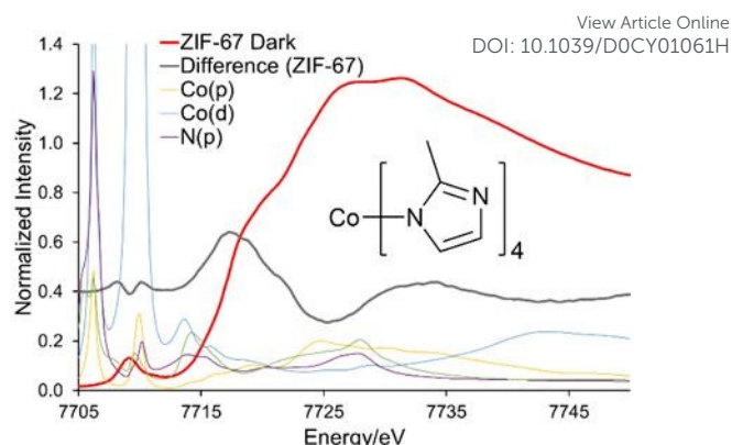
Fig. 4 DoS simulation results for ZIF-67, from the crystallographic structure of ZIF-67, showing the contributions from each orbital set. The difference spectrum is scaled by a factor of 20 and incremented by 0.4 for ease of observation.
