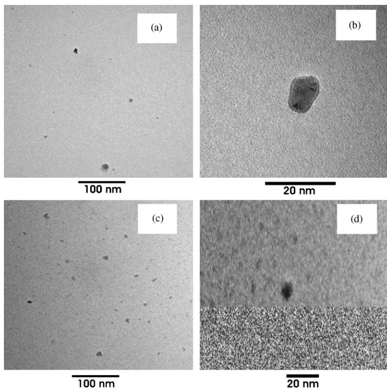
Fig. 2. TEM image of \text{CdFe}_2\text{O}_4 (a and b) and Cd (c and d) nanocrystals.
