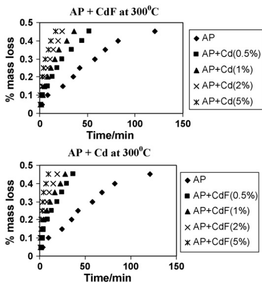
Fig. 6. Isothermal TG of AP with and without \text{CdFe}_2\text{O}_4 (CdF) and Cd nanocrystals on 300^\circ\text{C} .
