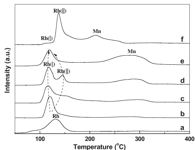
Fig. 4. The H_2 -TPR profiles of the Rh-Mn-Li/ \text{SiO}_2 catalysts with different Mn and Li amount: (a) 1.5Rh-0.075Li/ \text{SiO}_2 ; (b) 1.5Rh-0.5Mn-0.075Li/ \text{SiO}_2 ; (c) 1.5Rh-1Mn-0.075Li/ \text{SiO}_2 ; (d) 1.5Rh-1.5Mn-0.075Li/ \text{SiO}_2 ; (e) 1.5Rh-2.5Mn-0.075Li/ \text{SiO}_2 ; (f) 1.5Rh-1.5Mn-0.45Li/ \text{SiO}_2 .
