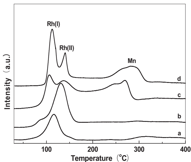
Fig. 3. The H_2 -TPR profiles of the different catalysts: (a) 1.5Rh/ \text{SiO}_2 ; (b) 1.5Rh-0.075Li/ \text{SiO}_2 ; (c) 1.5Rh-1.5Mn/ \text{SiO}_2 ; (d) 1.5Rh-1.5Mn-0.075Li/ \text{SiO}_2 .
