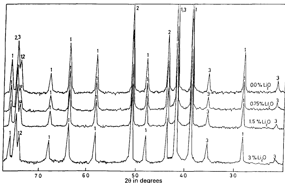
Fig. 6. X-ray diffractograms of basic \text{NiCO}_3:198(\text{Fe}_2\text{O}_3 \cdot 1.5\text{H}_2\text{O}) doped with \text{Li}_2\text{O} and calcined in air at 700^\circ\text{C} ; 1, \alpha\text{-Fe}_2\text{O}_3 ; 2, \text{NiO} ; 3, \text{NiFe}_2\text{O}_4 .
