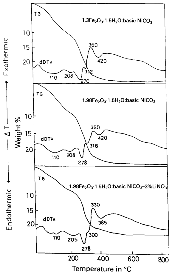
Fig. 3. TG, DTA and dDTA of different mixed solids.
