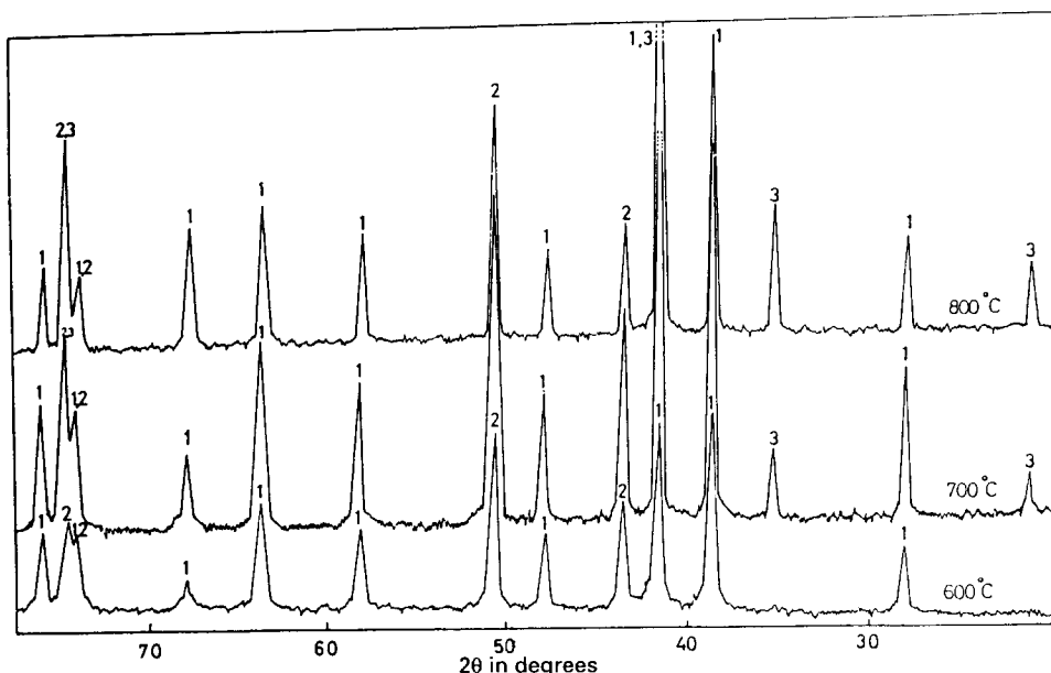
Fig. 5. X-ray diffractograms of basic \text{NiCO}_3:1.98(\text{Fe}_2\text{O}_3 \cdot 1.5\text{H}_2\text{O}) calcined in air at 600, 700 and 800°C; 1, \alpha\text{-Fe}_2\text{O}_3 ; 2, NiO; 3, \text{NiFe}_2\text{O}_4 .
