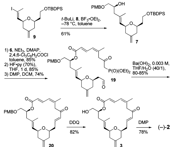
Scheme 4. Final Steps in the Total Synthesis of (–)- 2
