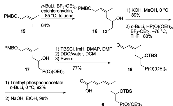
Scheme 3. Synthesis of Unsaturated Acid 6
