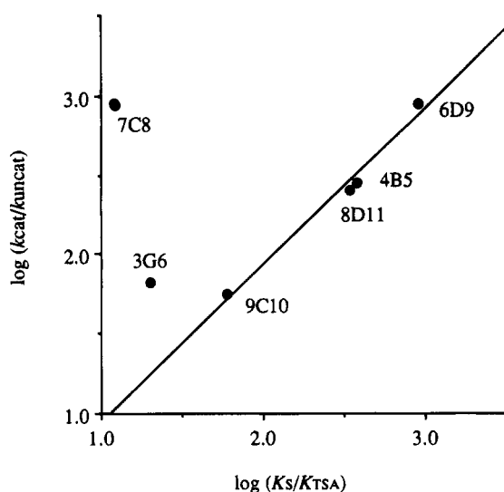
Figure 2. Plot of \log(K_S/K_{\text{TSA}}) versus \log(k_{\text{cat}}/k_{\text{uncat}}) for catalytic antibodies generated against phosphonate transition state analog 3 . A linear relationship was obtained for antibodies 6D9, 4B5, 8D11, and 9C10, suggesting that the antibody-combining sites act as catalysts by stabilizing the transition state; slope = 0.99, R^2 = 0.98 . Data represented in this figure are in Table 1.
