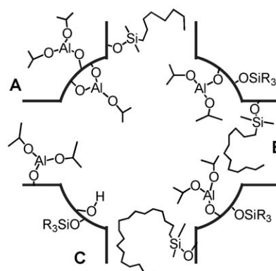
Scheme 2. Schematic representation of the cage-like pore structure of hybrid catalysts \text{Al}(\text{OiPr})_x\text{@SBA-1} (A), \text{Al}(\text{OiPr})_x\text{@SiMe}_2\text{C}_8\text{H}_{17}\text{@SBA-1} (B), and \text{Al}(\text{OiPr})_x\text{@SiMe}_2\text{C}_{18}\text{H}_{37}\text{@SBA-1} (C).
