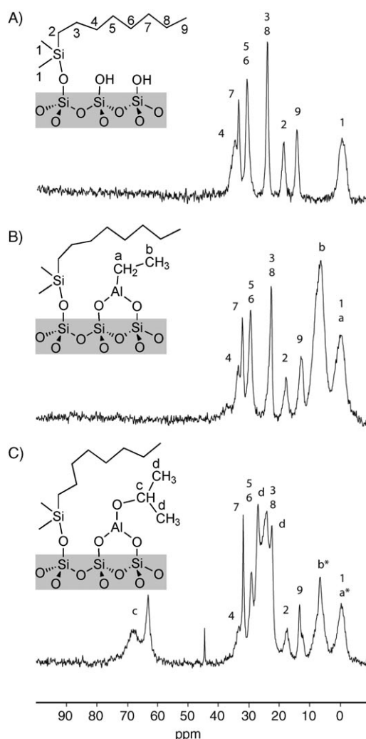
Figure 2. ^{13}\text{C} MAS NMR spectra of A) \text{SiMe}_2\text{C}_8\text{H}_{17}\text{@SBA-1} , B) \text{AlEt}_x\text{@SiMe}_2\text{C}_8\text{H}_{17}\text{@SBA-1} , and C) \text{Al}(\text{OiPr})_x\text{@SiMe}_2\text{C}_8\text{H}_{17}\text{@SBA-1} and schematic drawings of proposed surface species.
