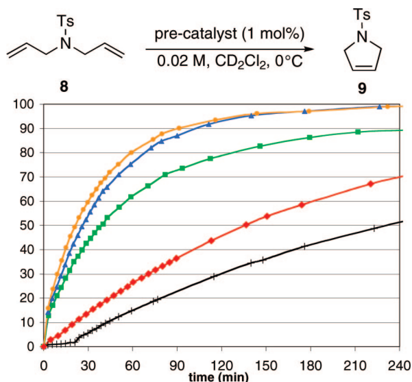
FIGURE 4. Kinetic studies of RCM of disubstituted olefin 8 (0.02 M) with commercially available precatalysts and 2h (1 mol %) in \text{CD}_2\text{Cl}_2 at 0 °C: ( 1 , +), ( 2a , ♦), ( 2c , ●), ( 2d , ▲), ( 2h , ■). Conversion determined by NMR spectroscopy.
