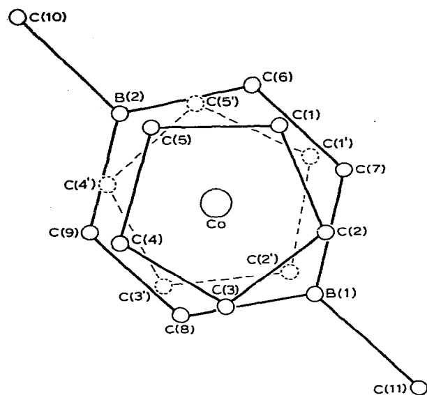
Fig. 2. Molecular structure of III seen in projection perpendicular to the plane of the cyclopentadienyl ring.
