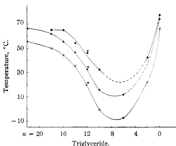
Fig. 4.—M.p. data for PC_nC_n series (data of Jackson, Lutton, et al. , except M-data of Malkin, et al. ): O, alpha (sub-alpha); \bullet , beta prime; \bullet , beta.
