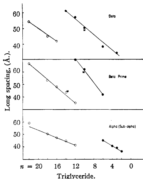
Fig. 5.—Long spacings for SC_nC_n series (data of Jackson, Lutton, et al. , except M-data of Malkin, et al. ): O, double chain length structure; \bullet , triple chain length structure.
