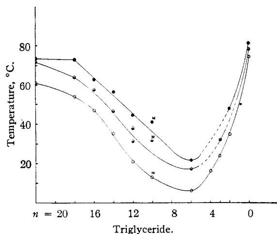
Fig. 3.—M.p. data for SC_nC_n series (data of Jackson, Lutton, et al. , except M-data of Malkin, et al. ): O, alpha (sub-alpha); \bullet , beta prime; \bullet , beta.
