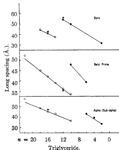
Fig. 6.—Long spacings for PC_nC_n series (data of Jackson, Lutton, et al. , except M-data of Malkin, et al. ): O, double chain length structure; \bullet , triple chain length structure.
