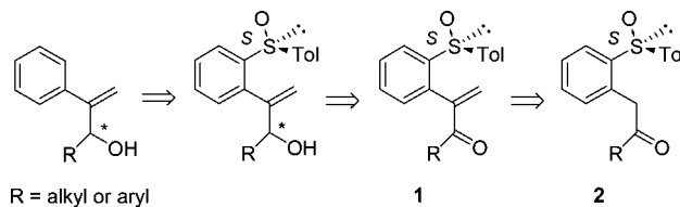
FIGURE 1. Retrosynthetic pathway of enantiomerically pure allylic carbinols.
