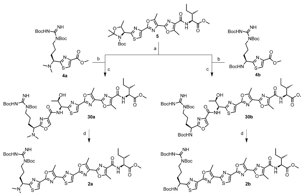
Scheme 6. a) HCl, 1,4-dioxane, RT, 1 h; b) LiOH, THF/H 2 O (1:1), 0 °C, 1.5 h; c) HATU, NiPr 2 Et, CH 2 Cl 2 , DMF, 0 °C → RT, 22 h, 61 % 30a , 66 % 30b ; d) Deoxo-Fluor, CH 2 Cl 2 , -20 °C, 2 h then BrCCl 3 , DBU, 0 °C, 20 h ( 2a )/15 h ( 2b ), 69 % 2a , 92 % 2b . DMF = N,N -dimethylformamide.
