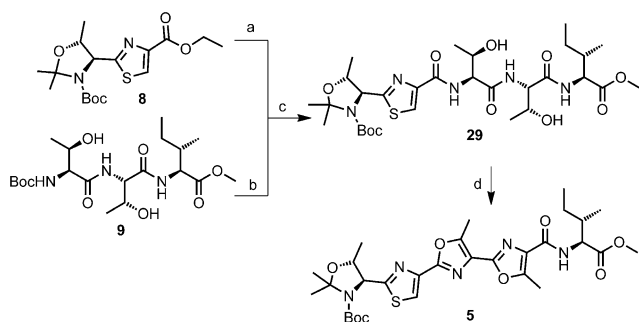
Scheme 5. Reagents and conditions: a) LiOH-H 2 O, MeOH/H 2 O (3:2), RT, 3 h; b) HCl, 1,4-dioxane, 30 min; c) HOBt, EDCI, NiPr 2 Et, CH 2 Cl 2 , RT, 18 h, 71 %, (3 steps); d) Deoxo-Fluor, CH 2 Cl 2 , -20 °C, 2 h, then BrCCl 3 , DBU (portionwise), 5 d, 0 °C, 64 %. Deoxo-Fluor = bis(2-methoxyethyl)aminosulfur trifluoride, DBU = 1,8-diazabicyclo-[5.4.0]undec-7-ene.
