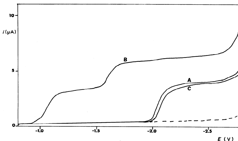
Fig. 1. Polarograms of 1 mmol 1 (curve A), (fluorenone) \text{Cr}(\text{CO})_3 (curve B) and 6 (curve C).
