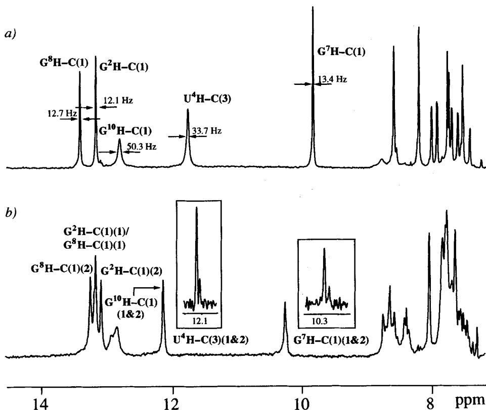
Fig. 9. 1D ^1H -NMR Spectra (600 MHz, H_2O ) of a) the unmodified 5'-r[CGC(UUCG)GCG]-3' and b) the 2'-fluorinated 5'-r[C f GC f (U f U f C f G)GC f G]-3' in the imino-resonance region 1)
