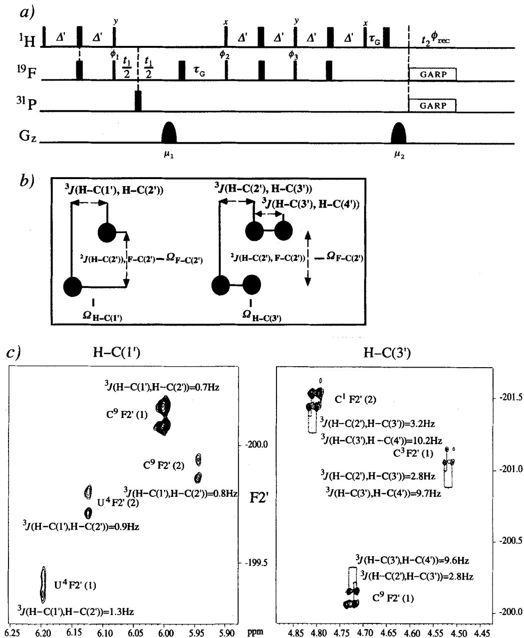
Fig. 12. a) Pulse sequence for the ^{19}\text{F}, ^1\text{H} -HSQC-E.COSY experiment. b) Schematic drawing of the expected cross-peak pattern (the \text{H-C}(1')/\text{F-C}(2') cross peak is splitted by ^3J(\text{H-C}(1'), \text{H-C}(2')) in \omega_2 and ^2J(\text{H-C}(2'), \text{F-C}(2')) in \omega_1 ; the F-atom is not affected during the back transfer of the magnetization, resulting in the indicated E.COSY splitting; the \text{H-C}(3')/\text{F-C}(2') cross peak is, in addition to splitting by ^3J(\text{H-C}(2'), \text{H-C}(3')) and ^2J(\text{H-C}(2'), \text{F-C}(2')) , split by the passive ^3J(\text{H-C}(3'), \text{H-C}(4')) in \omega_2 ). c) Experimentally obtained spectrum ( \text{F2}' = \text{F-C}(2')^1 )
