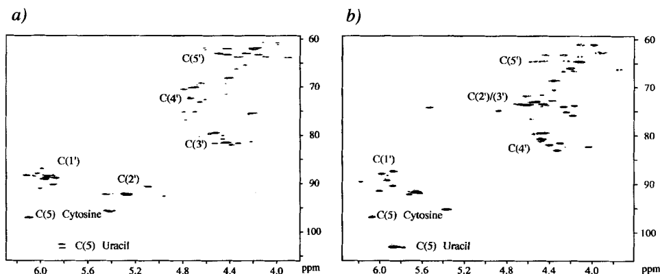
Fig. 4. Comparison of the ^1\text{H},^{13}\text{C} -HSQC spectra of a) the 2'-fluorinated 5'-r[ \text{C}_f\text{GC}_f(\text{U}_f\text{U}_f\text{C}_f\text{G})\text{GC}_f\text{G} ]-3' and b) the unmodified 5'-r[ \text{CGC}(\text{UUCG})\text{GCG} ]-3'. The overlap in the C(2')/C(3') region of the unmodified oligomer is overcome upon fluorination, the C(2') resonances in the C-dimension being shifted ca. 20 ppm downfield in the 2'-fluorinated oligomer.
