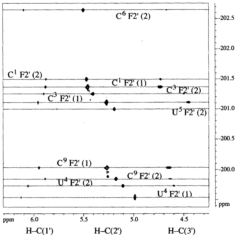
Fig. 6. ^1\text{H} , ^{19}\text{F} -HSQC Spectrum (600 MHz) of the 2'-fluorinated 5'-r[C f GC f (U f U f C f G)GC f G]-3'. The assignment of the fluorinated pyrimidine residues is indicated by horizontal dashed lines (F2' = F-C(2')). The respective conformation is given in parentheses (1 = hairpin, 2 = duplex).
