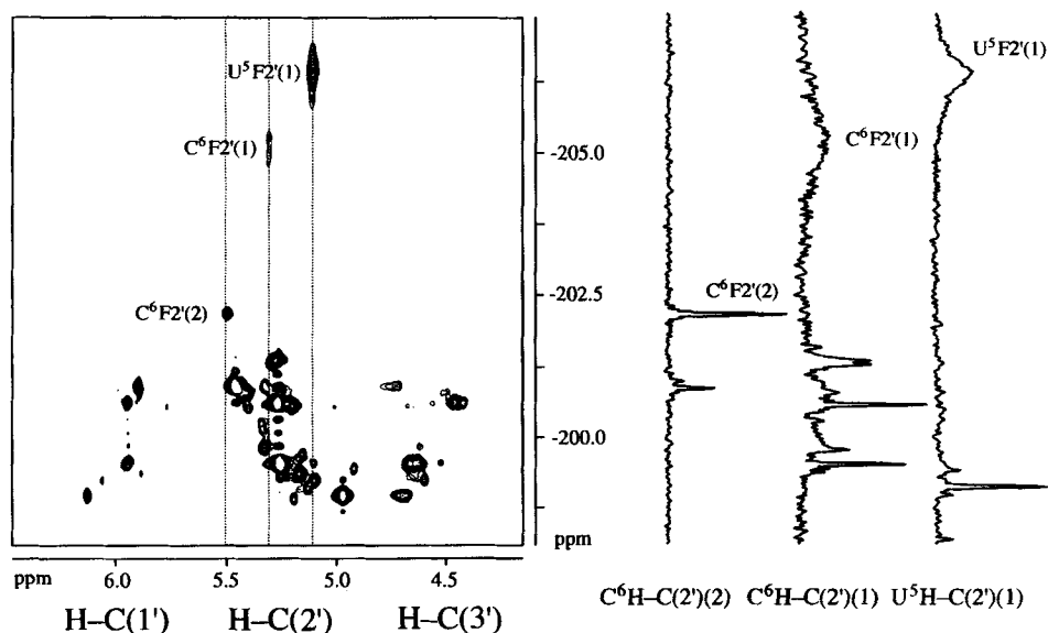
Fig. 7. 1 H, 19 F-HSQC Spectrum (400 MHz) of the 2'-fluorinated 5'-r[C 7 GC 7 (U 7 U 7 C 7 G)GC 7 G]-3'. In contrast to the same spectrum at 600 MHz (see Fig. 6), also the F-resonances of U 5 (1) and C 6 (1) are visible (F2' = F-C(2')). On the right, columns through resonances of C 6 H-C(2')(2), C 6 H-C(2')(1), and U 5 H-C(2')(1) are shown. Data were apodized using a line broadening of 20 Hz in the indirect dimension.
