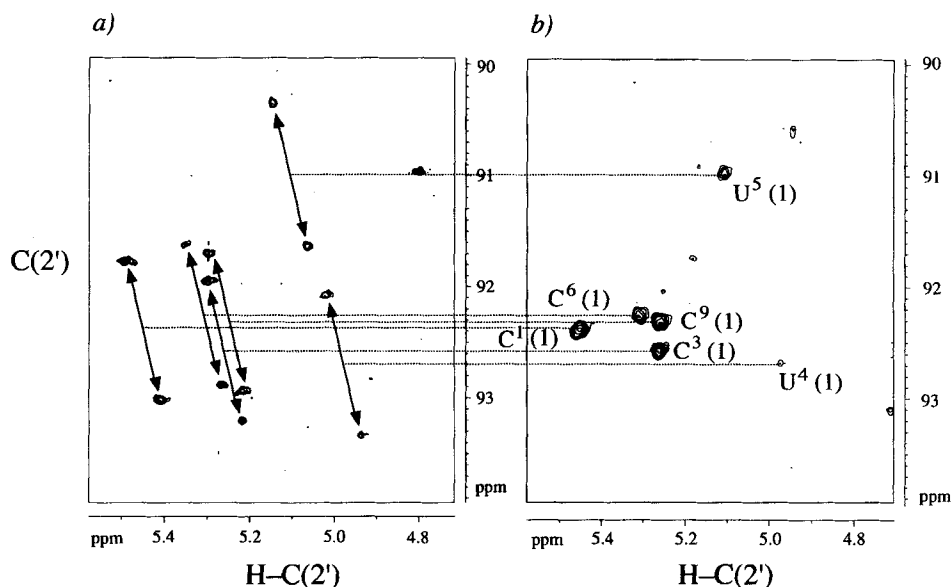
Fig. 5. ^1\text{H},^{13}\text{C} -HSQC Spectrum of the 2'-fluorinated 5'-r[ \text{C}_f\text{GC}_f(\text{U}_f\text{U}_f\text{C}_f\text{G})\text{GC}_f\text{G} ]-3' in the C(2')/H–C(2') region: a) without ^{19}\text{F} decoupling during t_1 and t_2 (at 600 MHz) and b) with decoupling of ^{19}\text{F} (at 400 MHz) 1) . Arrows indicate the E.COSY splitting of the peaks due to the F-atom which acts as a passive nucleus. This yields directly the ^2J(\text{H}–\text{C}(2'),\text{F}–\text{C}(2')) coupling constants in \omega_2 and ^1J(\text{C}(2'),\text{F}–\text{C}(2')) coupling constants in \omega_1 , respectively ^3J(\text{H}–\text{C}(1'),\text{F}–\text{C}(2')) and ^2J(\text{C}(1'),\text{F}–\text{C}(2')) (not shown). Numbers in parantheses after the nucleoside symbol indicate the conformation of the molecule (1 = hairpin, 2 = duplex).
