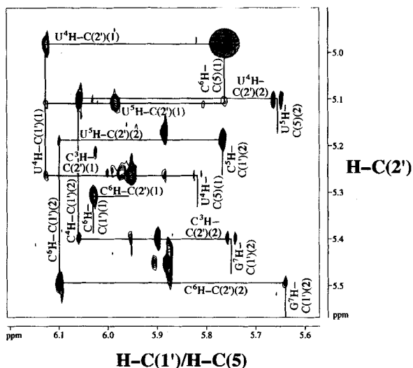
Fig. 10. NOESY Spectrum of the 2'-fluorinated 5'-r[C f GC f (U f U f C f G)GC f G]-3' in the H–C(1')/H–C(2') region 1 ). The U^4\text{H}-\text{C}(2')(1)/C^6\text{H}-\text{C}(5)(1) cross peak is highlighted in grey.
