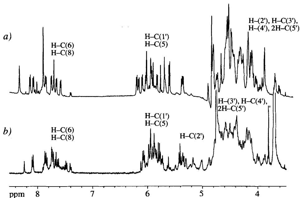
Fig. 3. Comparison of the 1D 1 H-NMR spectra (600 MHz) of a) the unmodified 5'-r[CGC(UUCG)GCG]-3' and b) the 2'-fluorinated 5'-r[C F GC F (U F U F C F G)GC F G]-3'. The H–C(2') resonances of the 2'-deoxy-2'-fluororibose moieties are clearly separated from the H–C(1') and H–C(2'), H–C(3'), H–C(4'), 2H–C(5') resonances of the ribose moieties.
