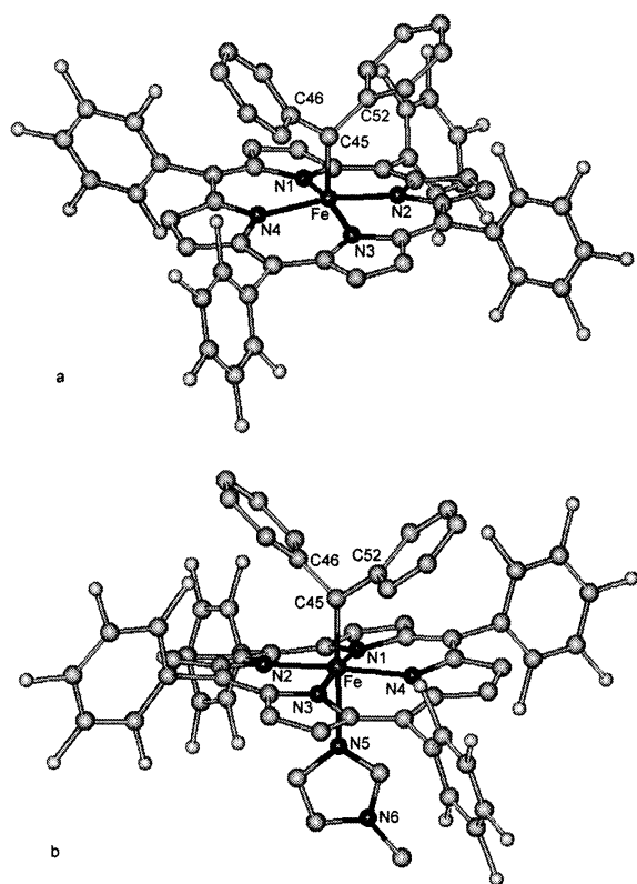
Figure 2. Ball and stick drawings of the structures of (a) [\text{Fe}(\text{TPFPP})(\text{CPh}_2)] \cdot 0.5\text{C}_6\text{H}_6 \cdot 0.5\text{CH}_2\text{Cl}_2 ( 1 ) and (b) [\text{Fe}(\text{TPFPP})(\text{CPh}_2)(\text{MeIm})] ( 4 ). The solvent molecules and/or hydrogen atoms are not shown.
