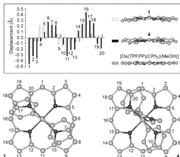
Figure 3. Orientations of the carbene axial ligands in [Fe(TPFPP)(CPh 2 )] ( 1 ) and [Fe(TPFPP)(CPh 2 )(Melm)] ( 4 ) with respect to the porphyrin ligands. The inset shows the perpendicular displacements of the porphyrin ring carbon atoms from the mean plane of the 24 component atoms (including four pyrrole nitrogens) observed for 1 , 4 , and the closely related osmium analogue [Os(TPFPP)(CPh 2 )(MeOH)] reported in ref 11, together with the side views of the porphyrin rings in these monocarbene complexes. The perpendicular displacements of the porphyrin ring nitrogen atoms from the mean plane of the 24 component atoms average 0.058 Å for 1 , 0.049 Å for 4 , and 0.041 Å for [Os(TPFPP)(CPh 2 )(MeOH)].
